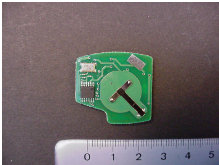
Picture 4 : vehicle remote keyless entry transmitter, view to the PCB, bottom side
