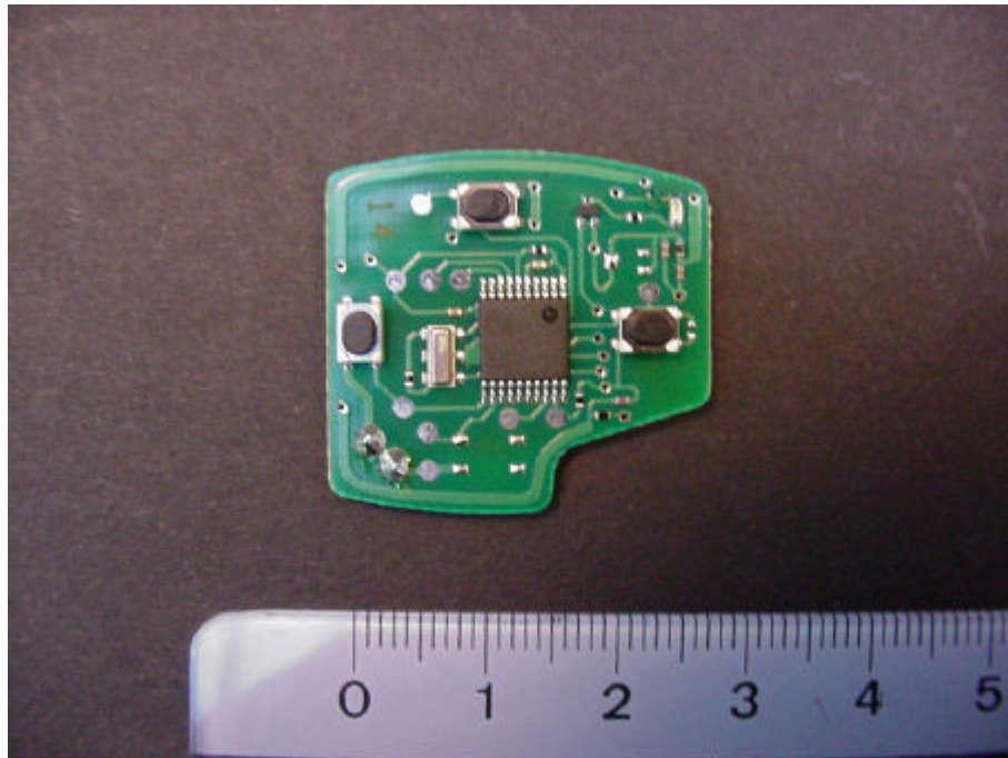
Picture 3 : vehicle remote keyless entry transmitter, view to the PCB, top side
