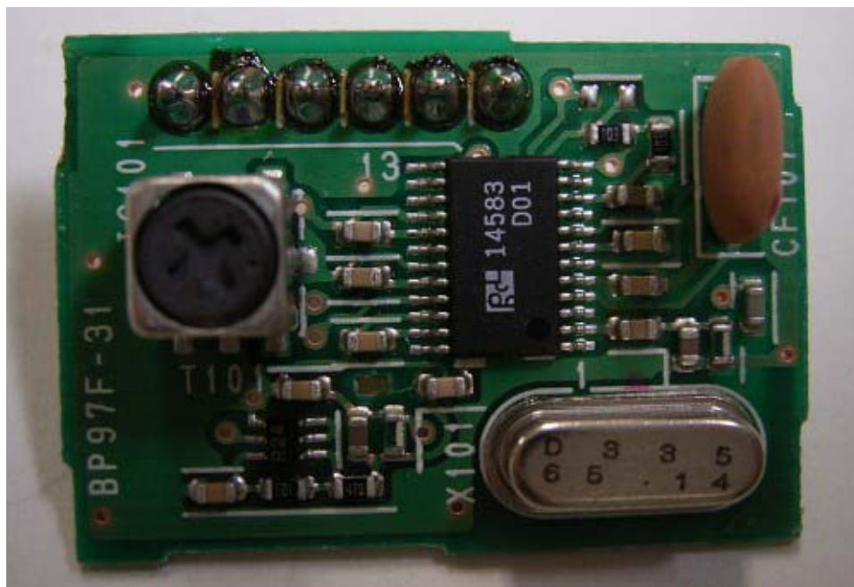
Tuner – Front without shield
