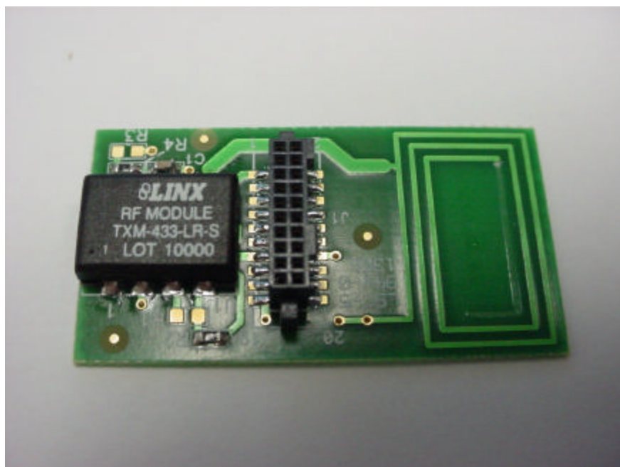
Top view of the Linx RF Module
