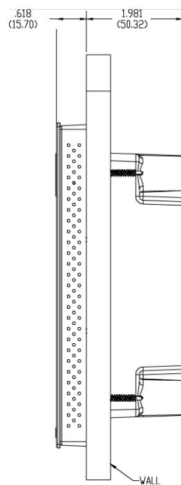
FIG. 40 MXD-1001 Installation Dimensions (side view)
