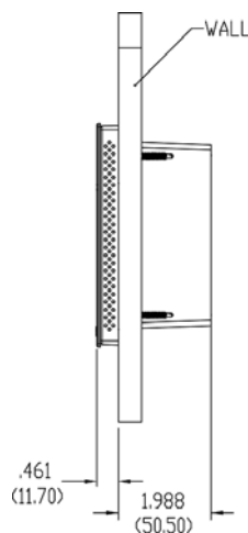
FIG. 43 MXD-700 Installation Dimensions (side view)
