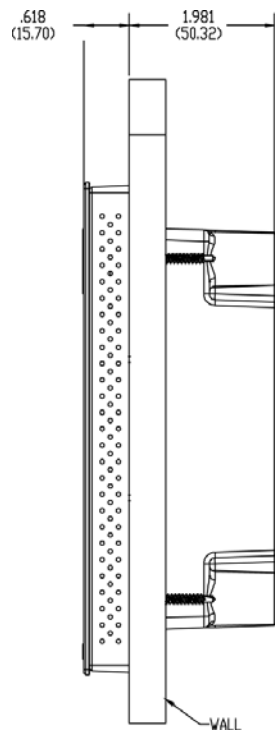
FIG. 41 MXD-1000 Installation Dimensions (side view)
