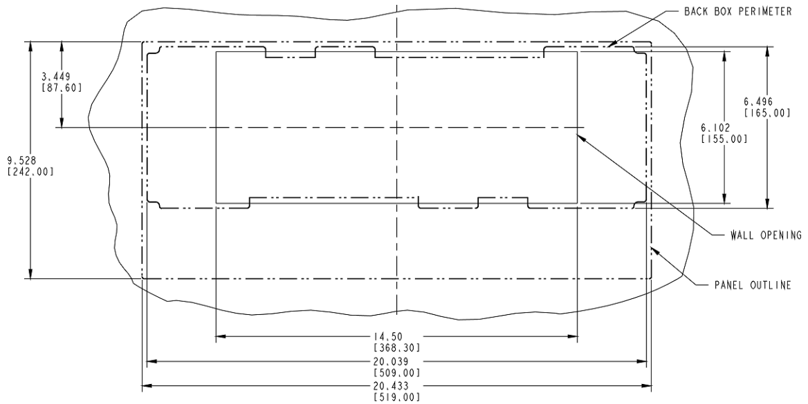
FIG. 27 MXD-2000XL-PAN-L Installation Dimensions (front view)
