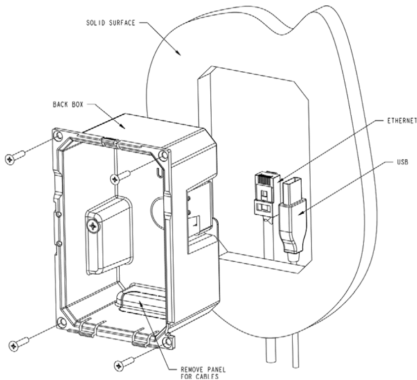
FIG. 55 MXD-430 Backbox Installation - Solid Surface
