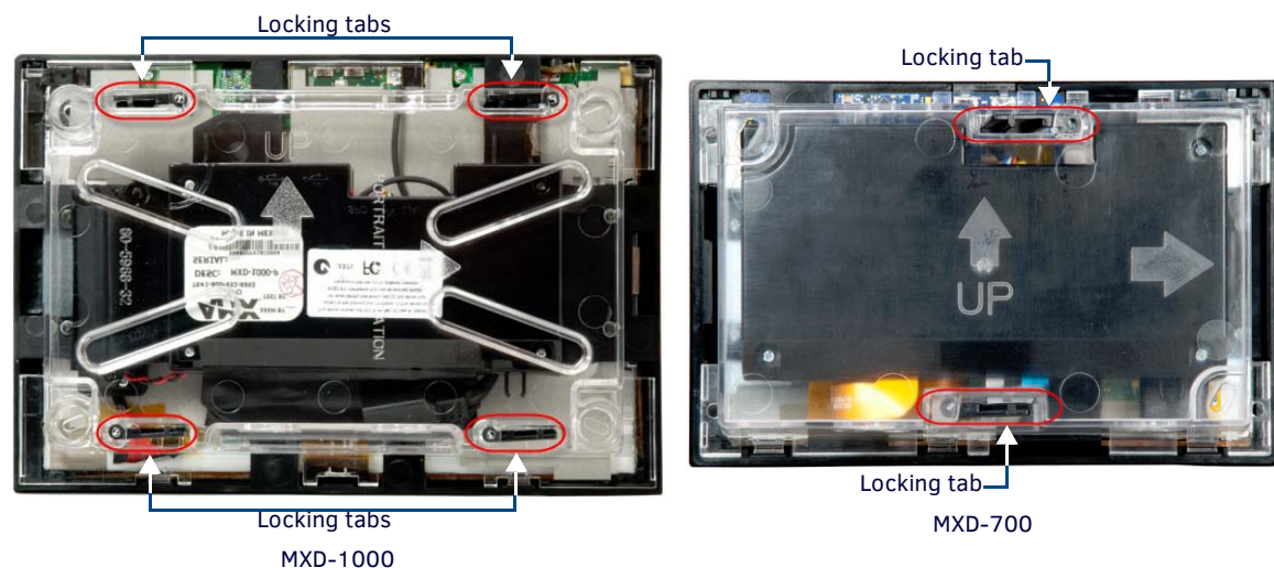
FIG. 36 MXD-1000 and MXD-700 Backboxes (Landscape orientation)
