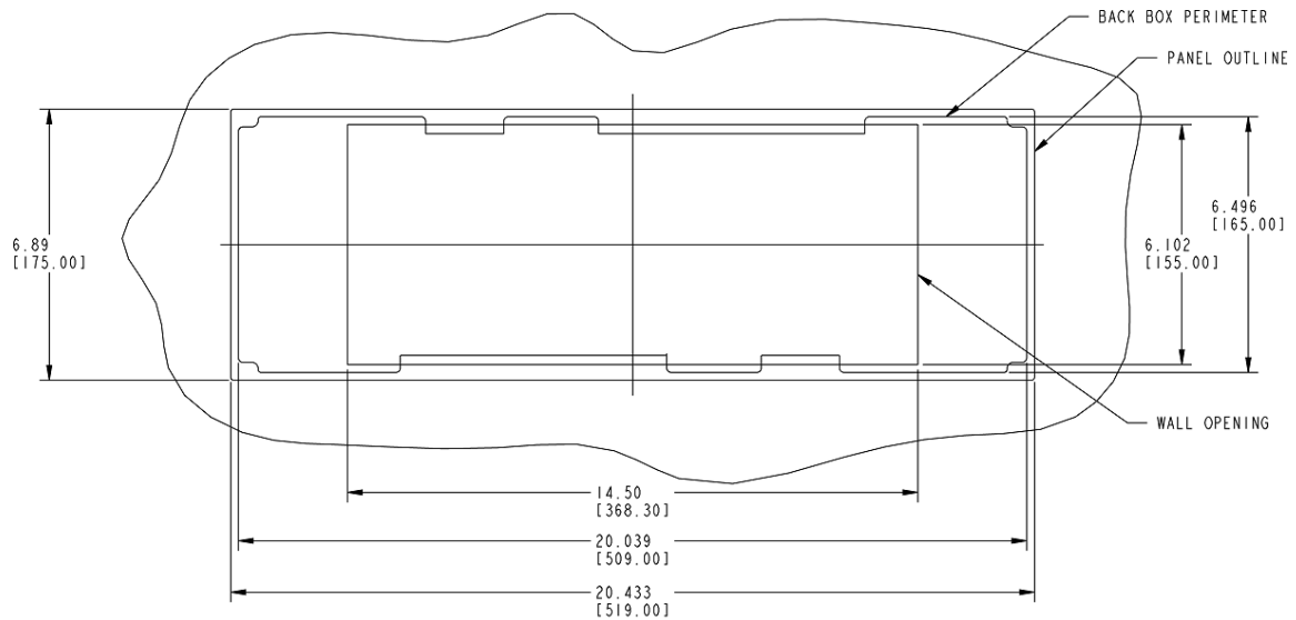
FIG. 29 MXD-1900L-PAN-L Installation Dimensions (front view)
