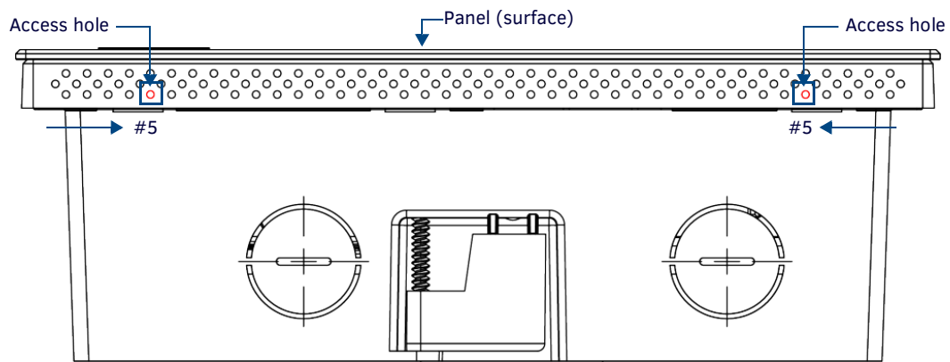
FIG. 51 Bottom View (Landscape) or Right-Side View (Portrait) of the MXD-700 showing access holes in molding
