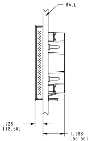
FIG. 30 MXD-1900L-PAN-L Installation Dimensions (side view)
