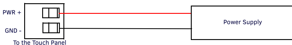
FIG. 19 NetLinx power connector wiring diagram
