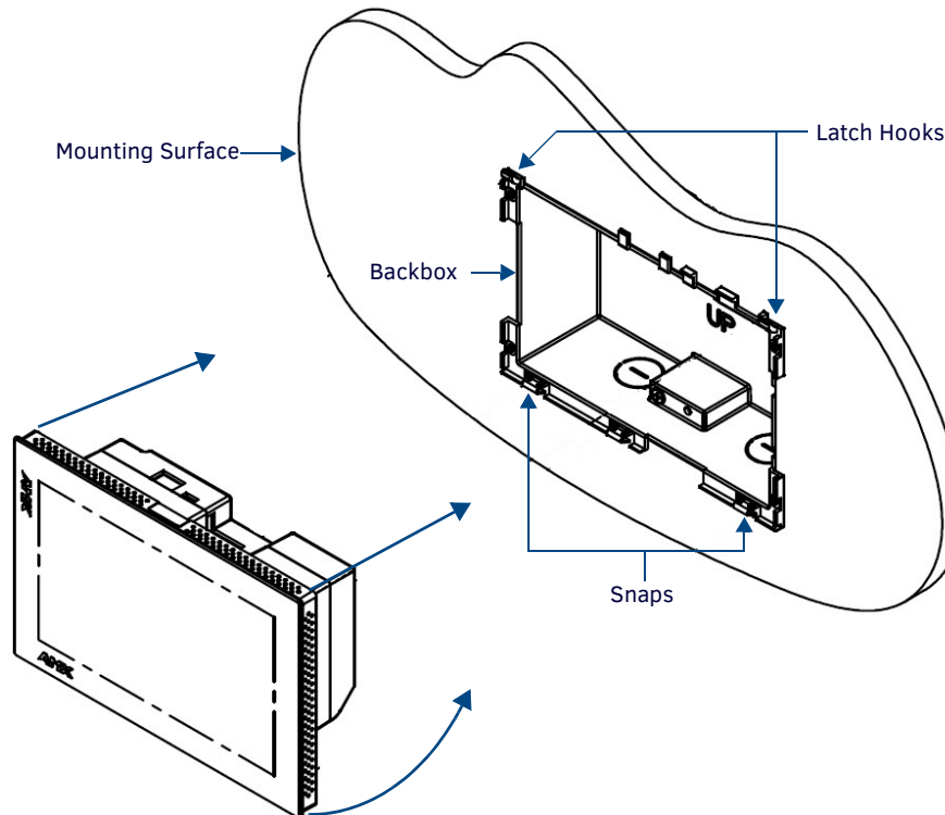
FIG. 46 Installing the MXD-1000 / MXD-700
