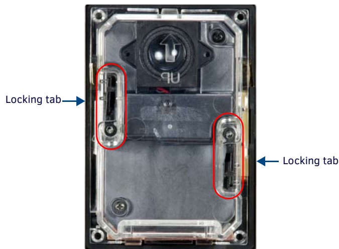
FIG. 52 MXD-430 Backbox
