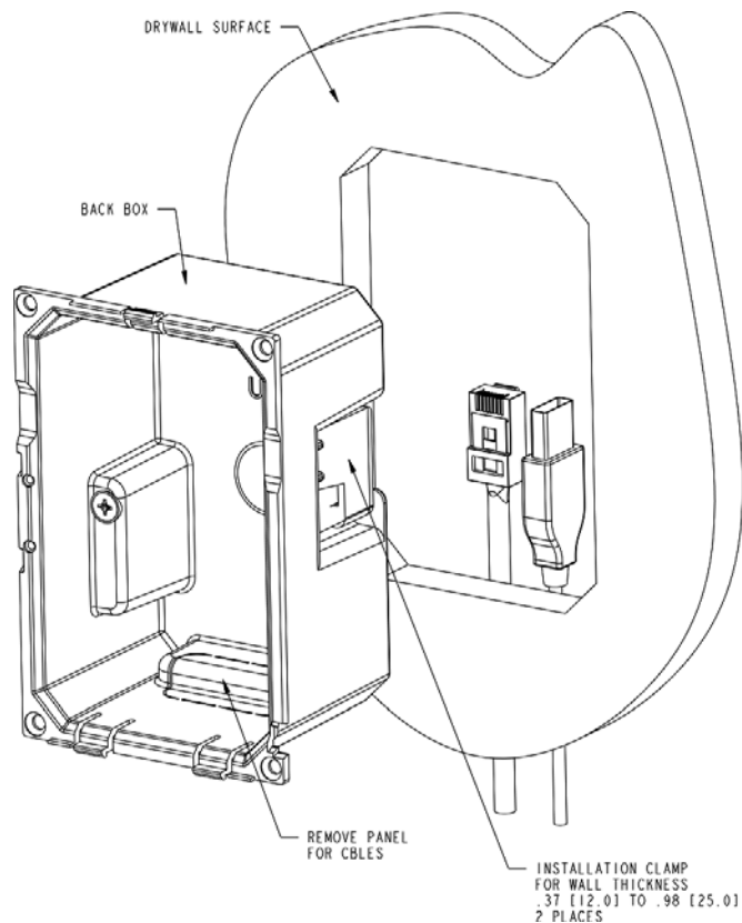
FIG. 56 MXD-430 Backbox Installation - Drywall Surface
