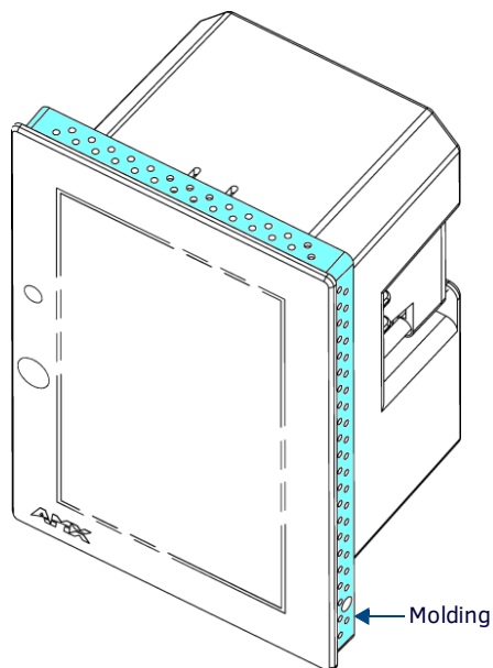
FIG. 59 MXD-430 Molding (highlighted in blue)
