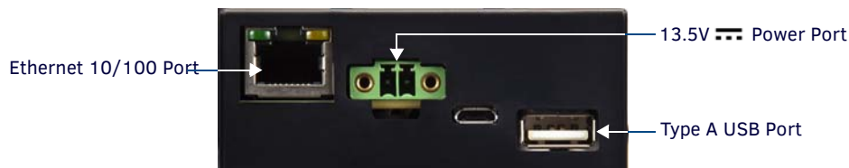
FIG. 16 MXT-2000XL-PAN / MXT-1900L-PAN - underside connectors
