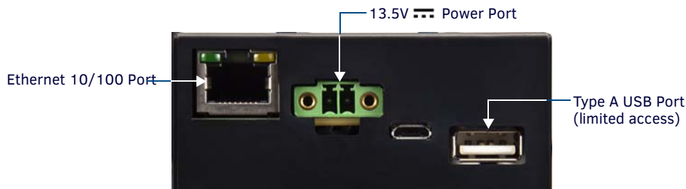
FIG. 32 MXD-2000XL-PAN / MXD-1900L-PAN - rear connectors
