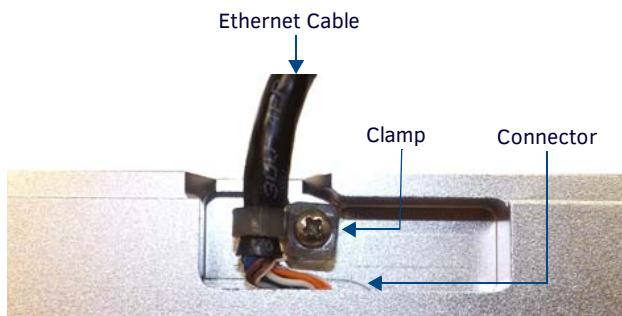
FIG. 20 Bottom of the MXT-700/1000
