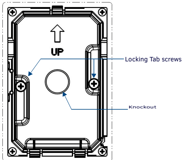
FIG. 57 MXD-430 Backbox installed in wall
