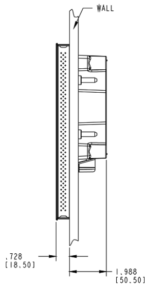
FIG. 28 MXD-2000XL-PAN-L Installation Dimensions (side view)
