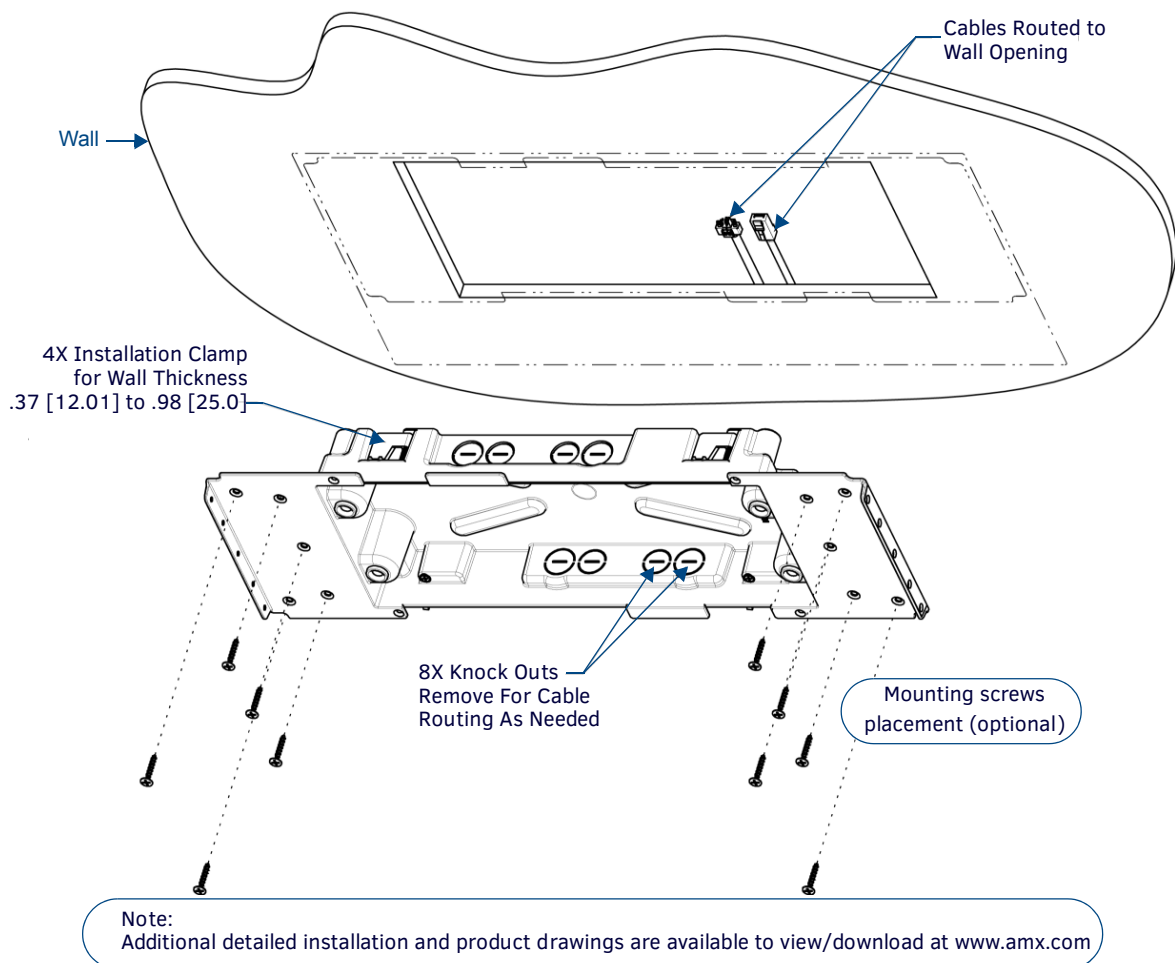
FIG. 31 MXD-1900L-PAN Backbox installation (Landscape)
