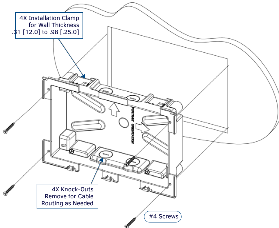
FIG. 44 MXD-1000 Backbox Installation (Landscape)
