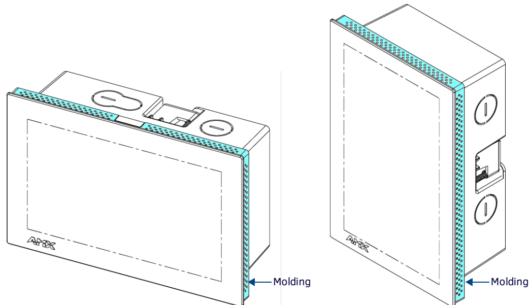
FIG. 50 MXD-700 Molding (highlighted in blue)
