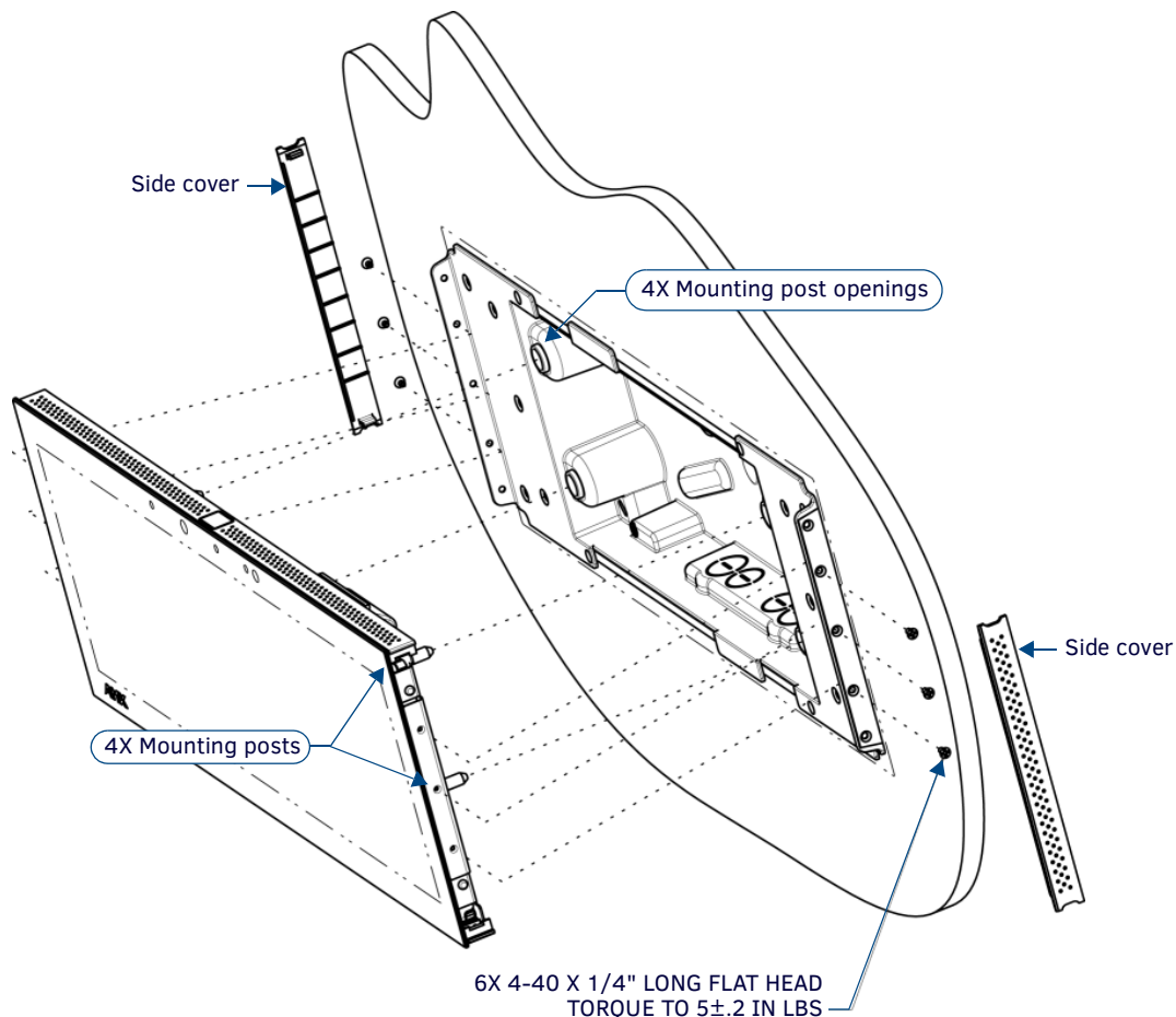
FIG. 33 MXD-1900L-PAN installation (Landscape)
