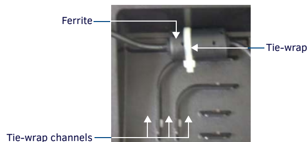
FIG. 17 Tie-wrap for power connector ferrite
