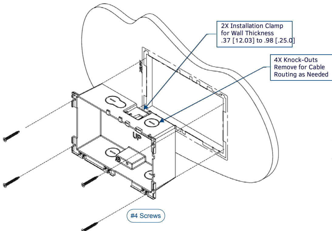
FIG. 45 MXD-700 Backbox Installation (Landscape)
