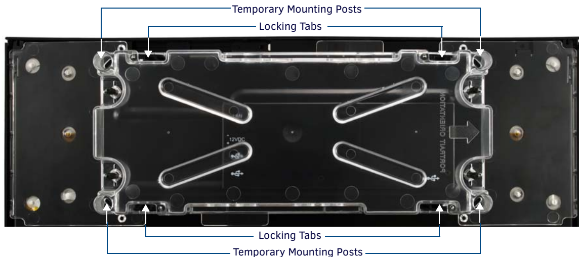
FIG. 23 Backbox (MXD-2000XL-PAN / MXD-1900L-PAN)
