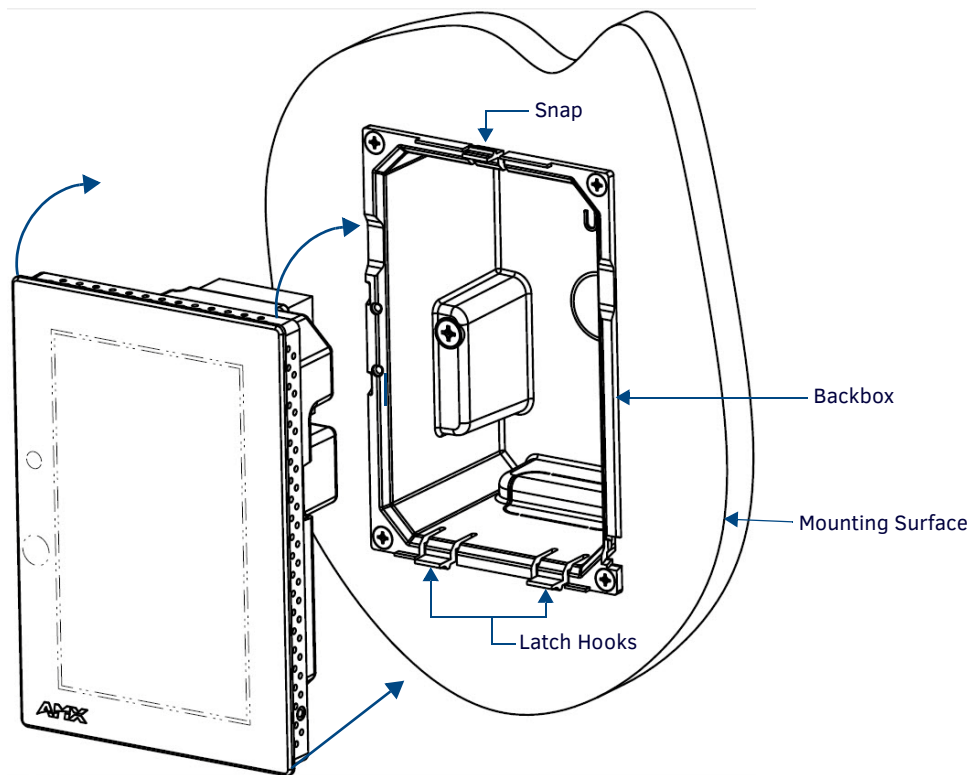
FIG. 58 Installing the MXD-430
