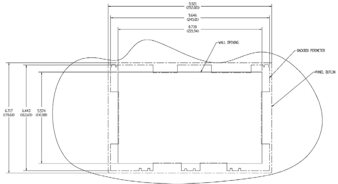
FIG. 40 MXD-1000 Installation Dimensions (front view)
