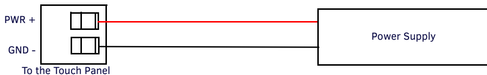
FIG. 34 NetLinX power connector wiring diagram
