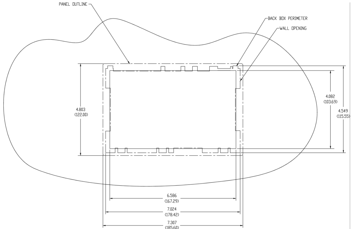
FIG. 42 MXD-700-L Installation Dimensions (front view)
