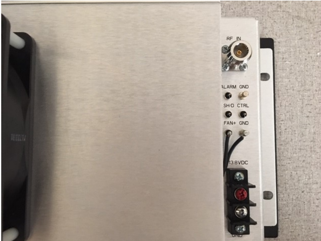
Left side view – connectors
