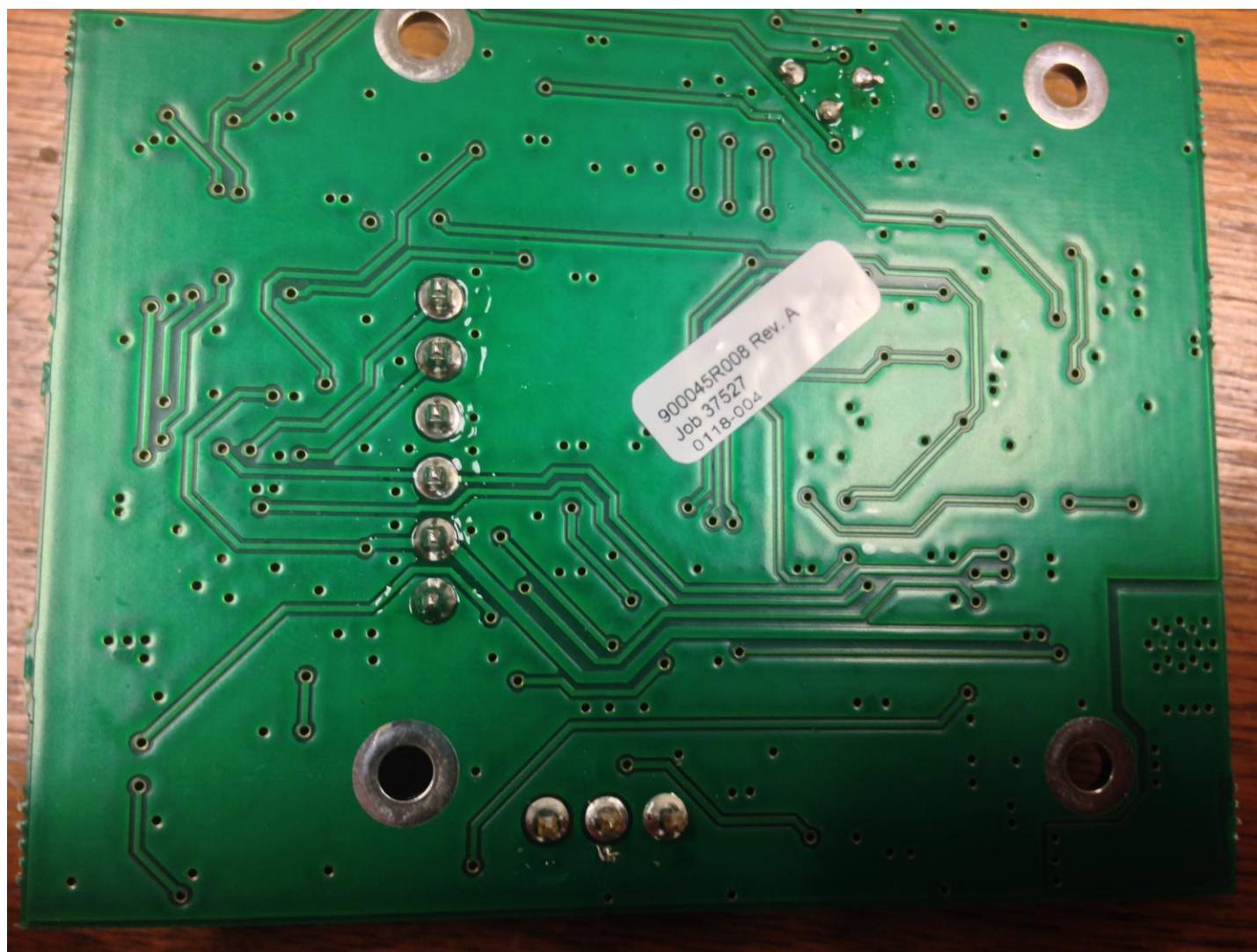
Control Board - Bottom
