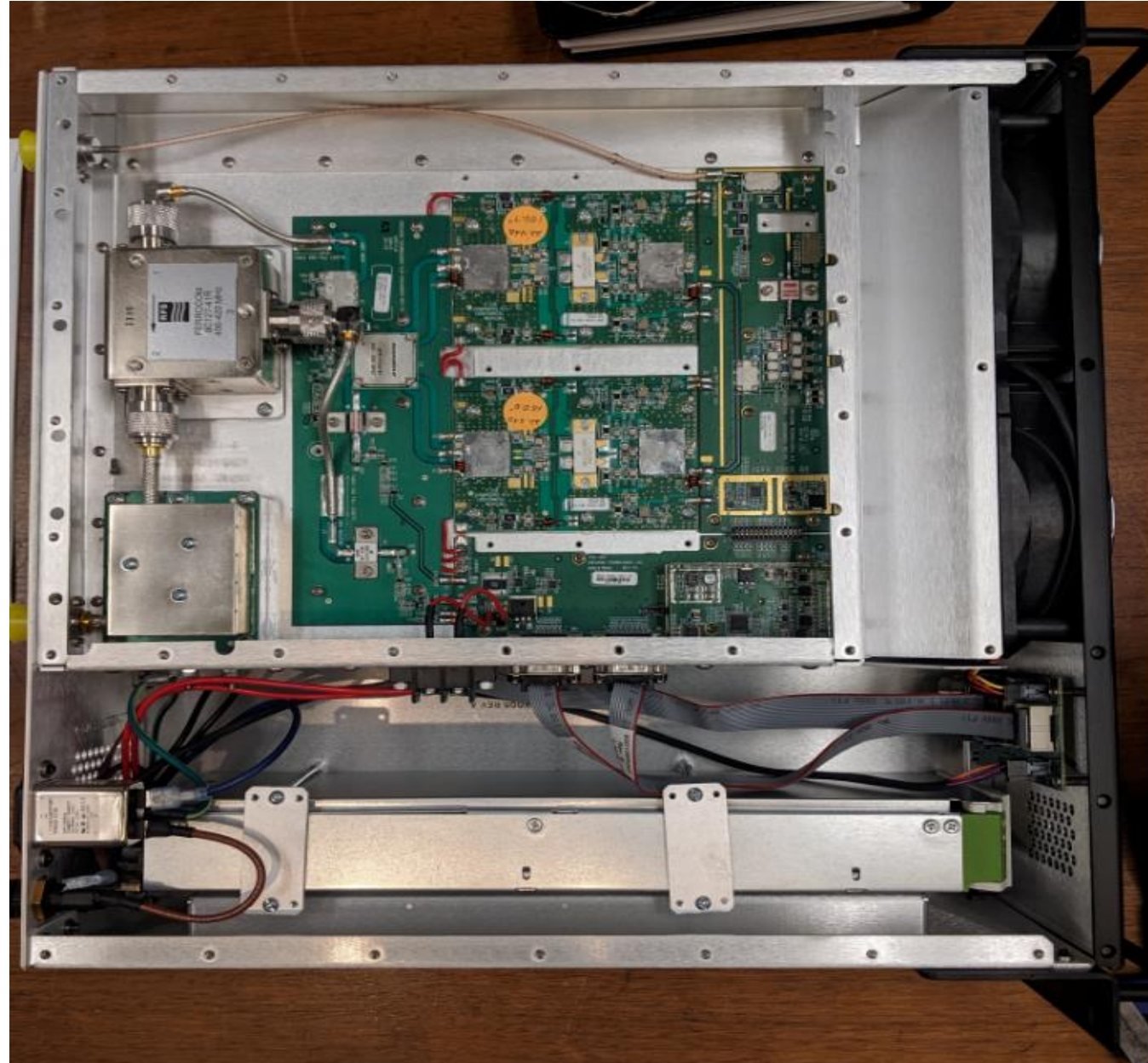
P25 UHF Low Band (406 – 420MHz) Full Amplifier
