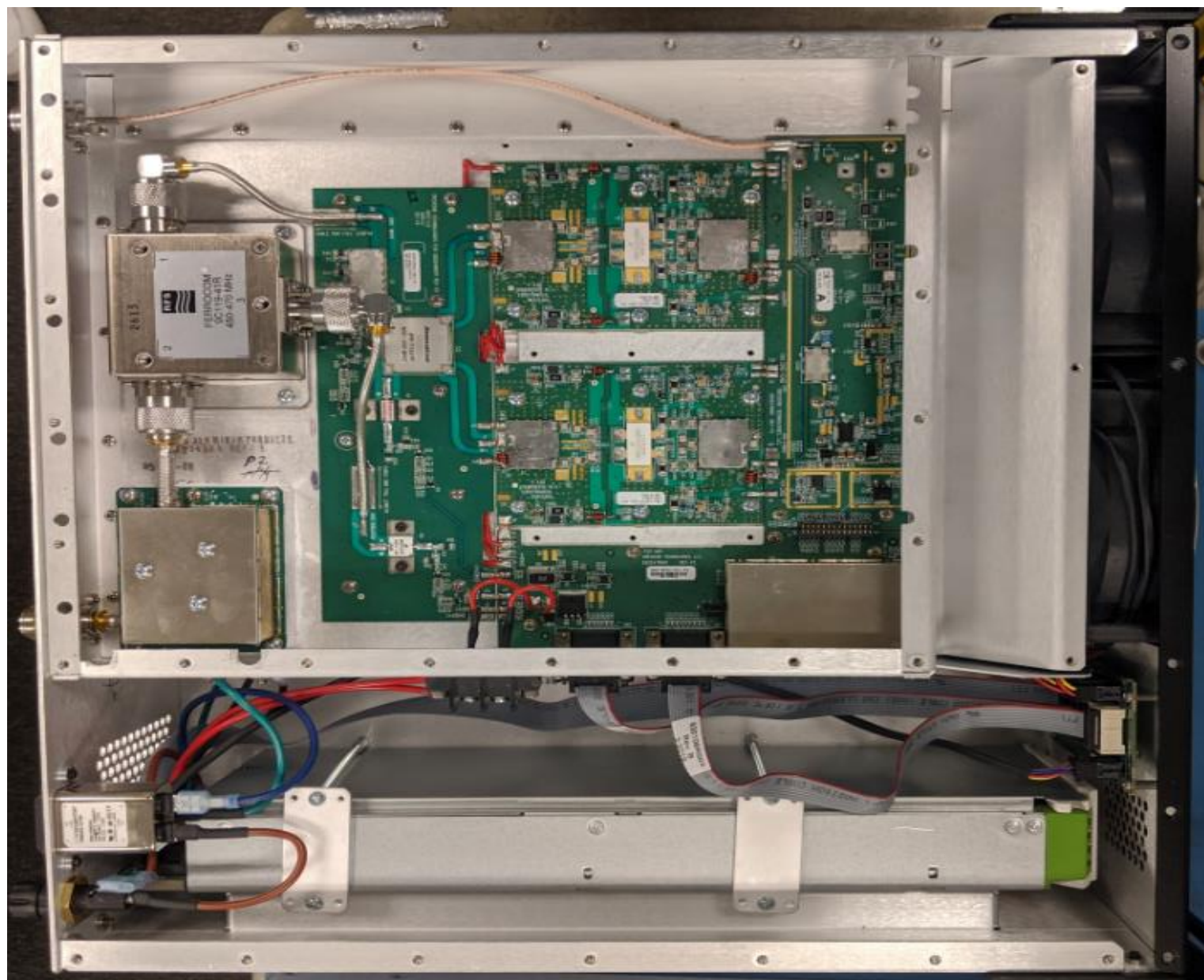
P25 UHF High Band (450-454MHz, 456-462.5375MHz, 462.7375-467.5375MHz, 467.7375-470 MHz) Pallet Board Top Side
