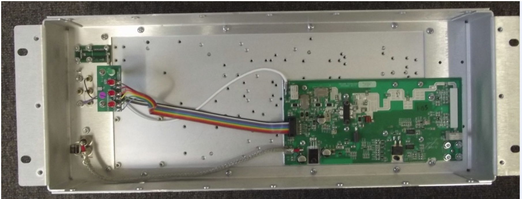
Unit – inside view
