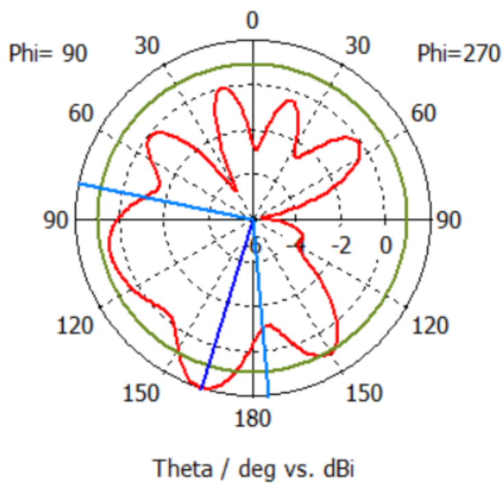
Farfield Directivity Abs (Phi=90)
