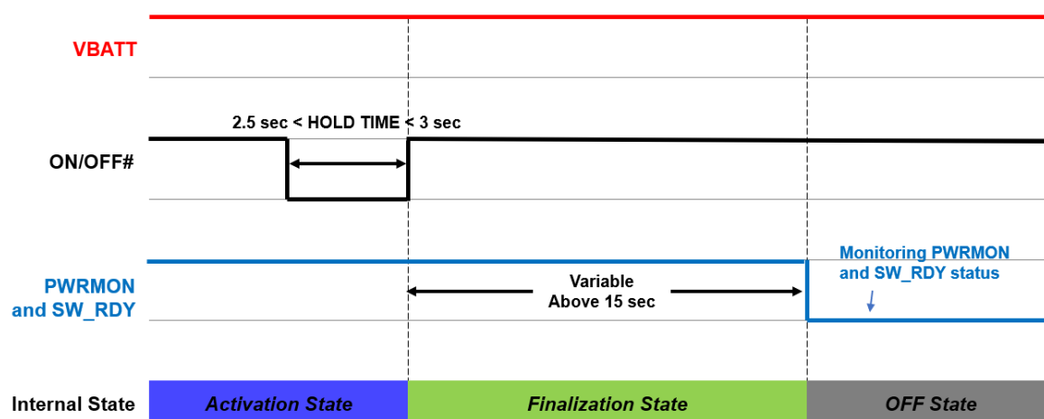
Figure 7: Hardware Shutdown
