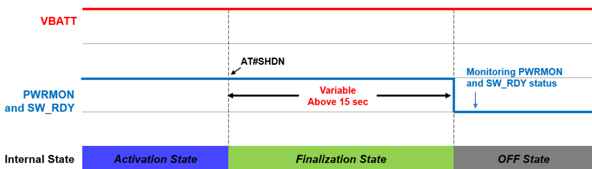
Figure 6: Shutdown by Software Command
