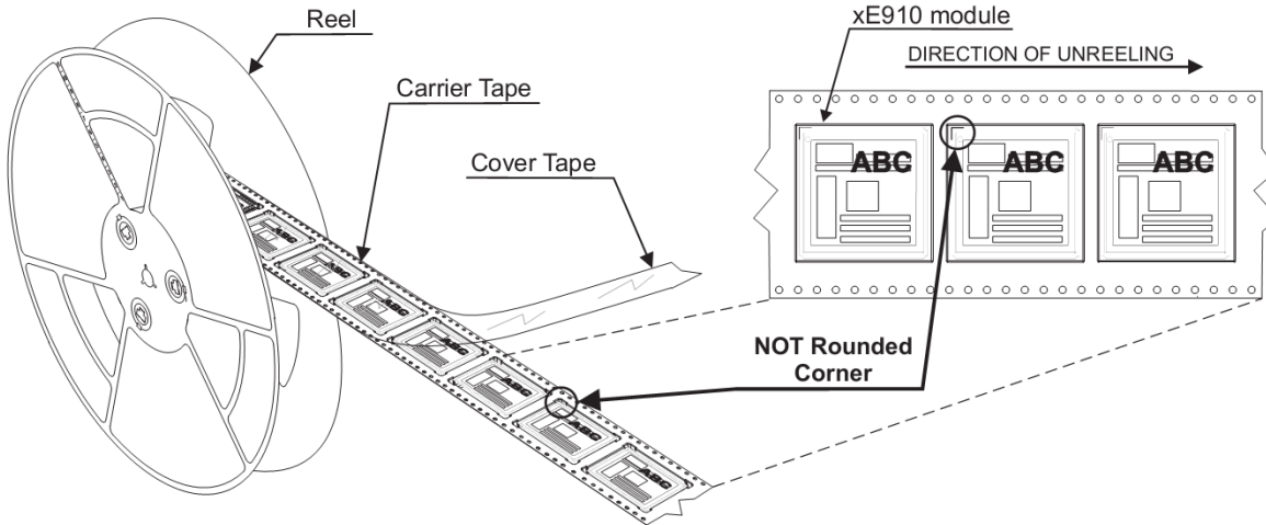
Figure 35: Carrier Tape Detail
