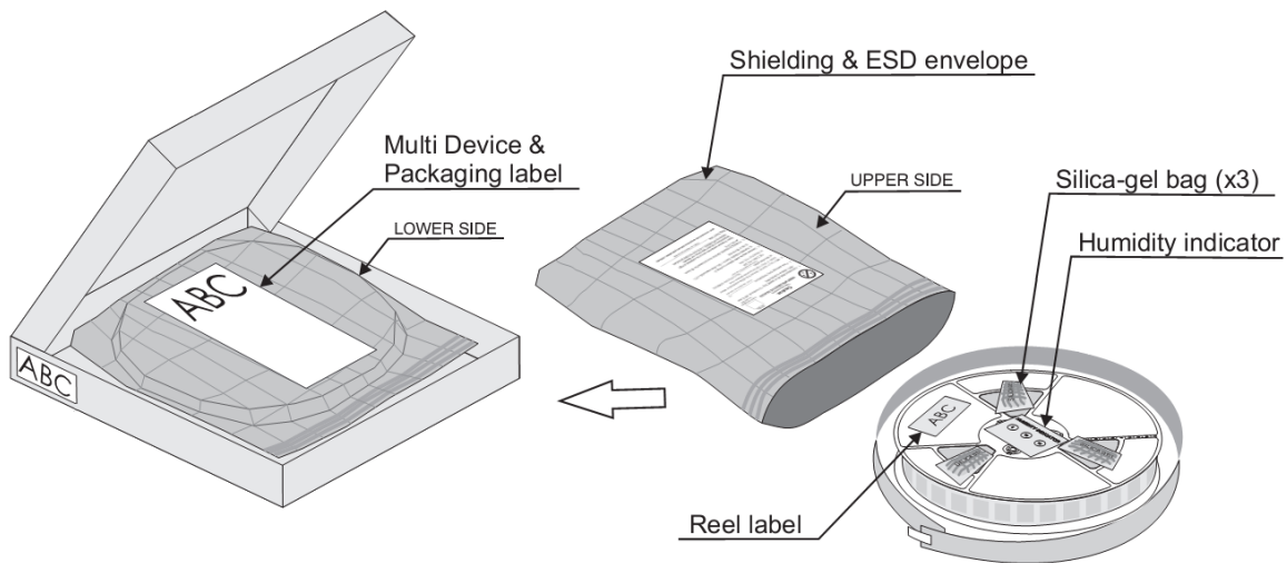
Figure 37: Reel Box Detail
