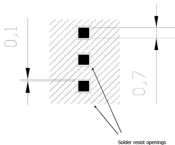
Figure 29: PCB Pad Dimensions
