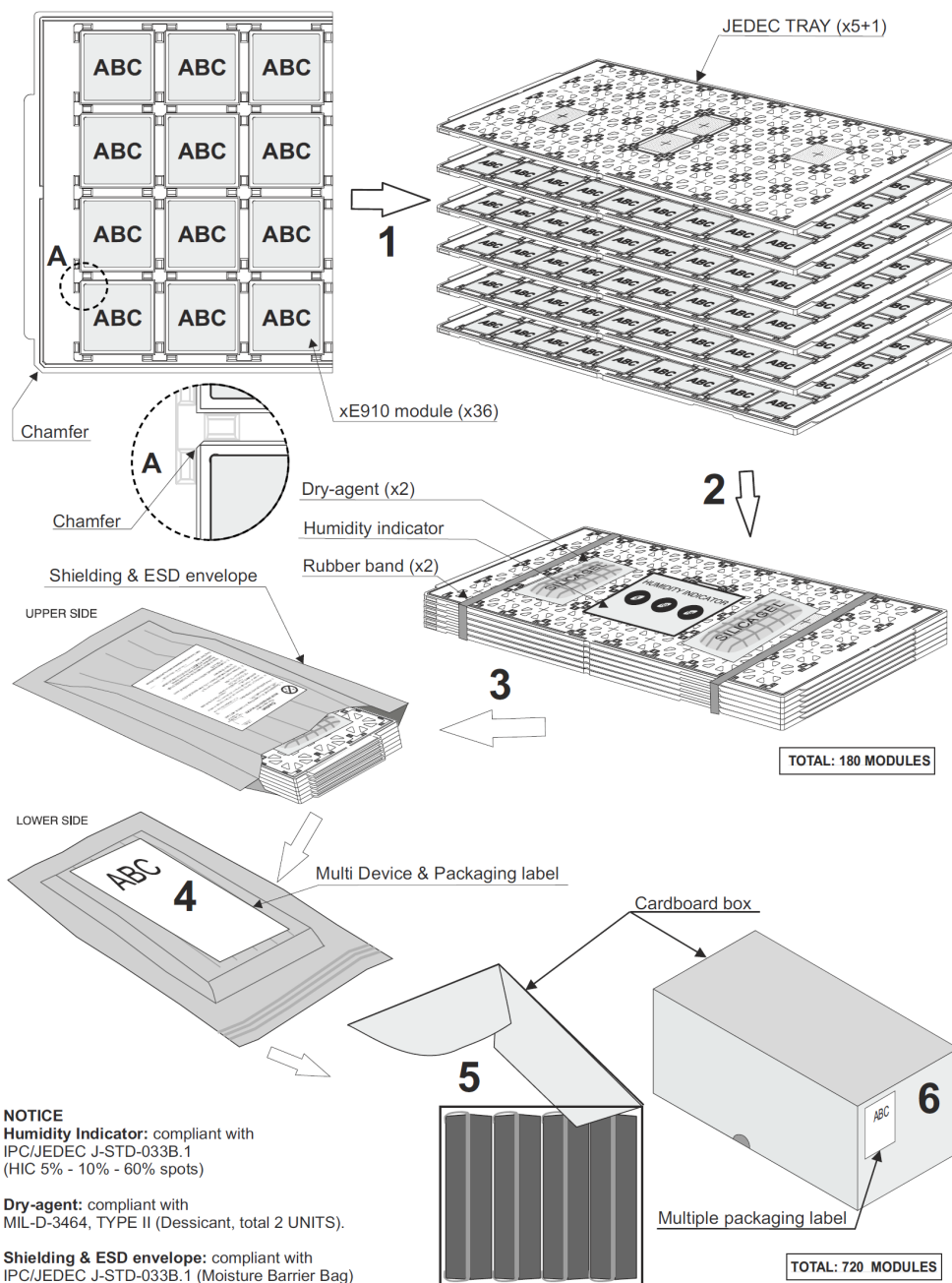
Figure 32: Packing
