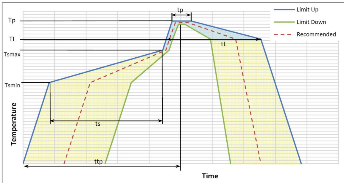
Figure 30: Solder Reflow Profile
