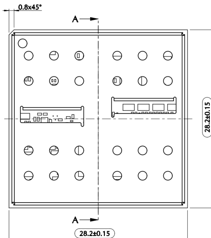
Figure 24: LE910Cx-SV/LA Mechanical Dimensions (Top view)
