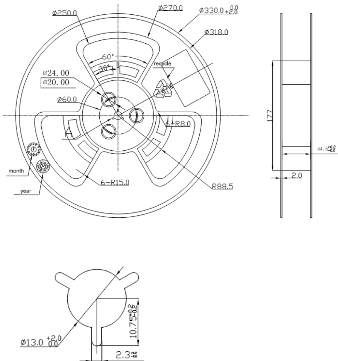
Figure 36: Reel Detail
