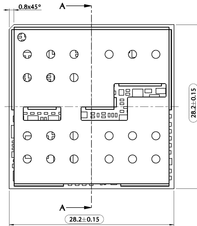
Figure 24: LE910Cx-SV/LA Mechanical Dimensions (Top view)
