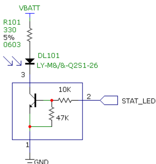
Figure 21: Status LED Circuit Example
