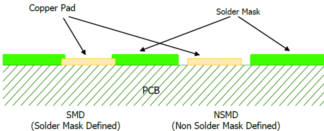
Figure 28: PCB Pad Design
