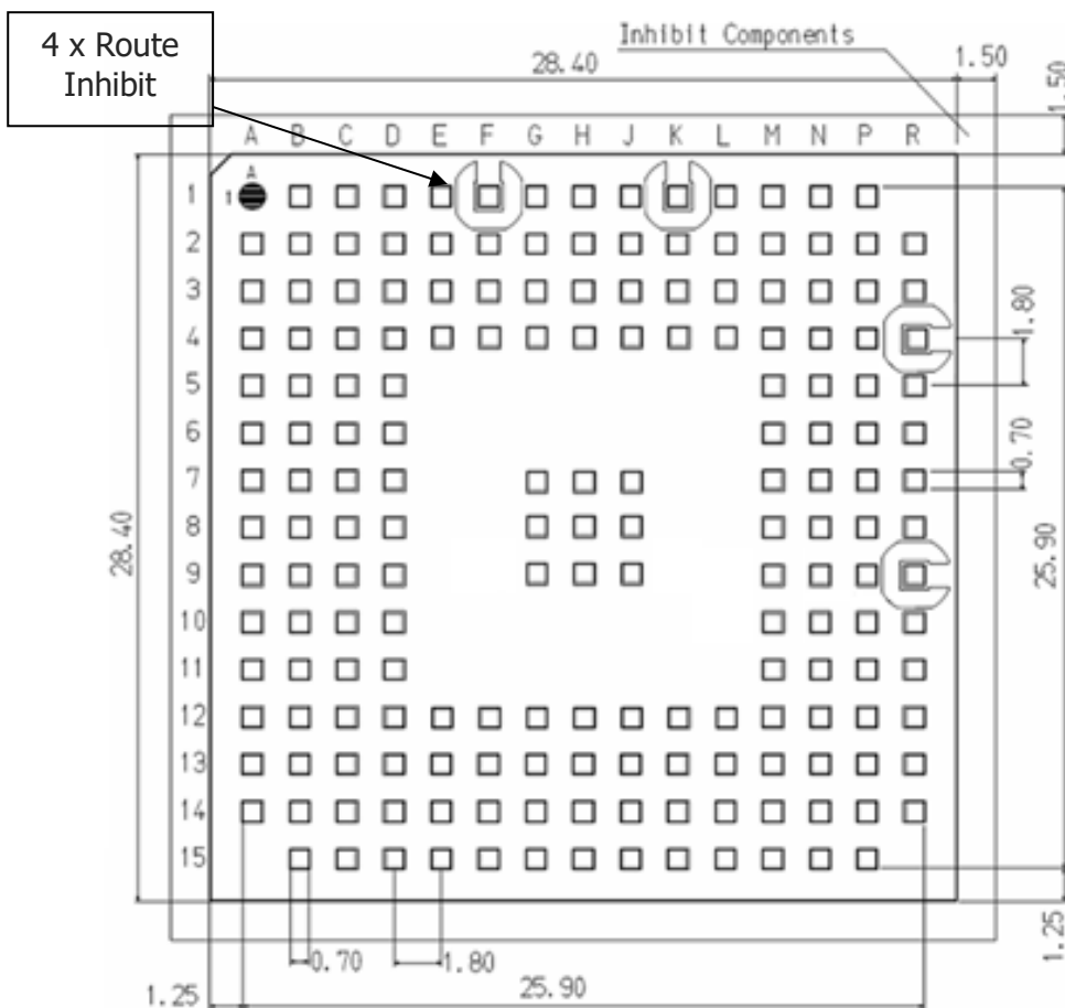
Figure 27: Recommended Footprint - Top View, 181 pads
