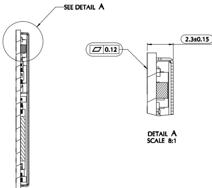
Figure 26: LE910C1-SV Mechanical Dimensions (Side view)
