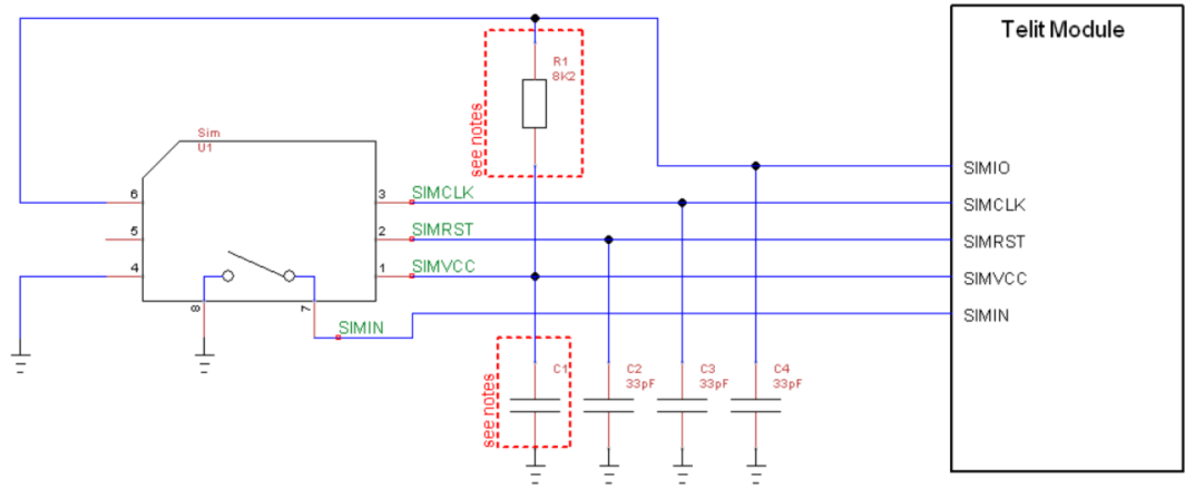
Figure 31: SIM Schematics
