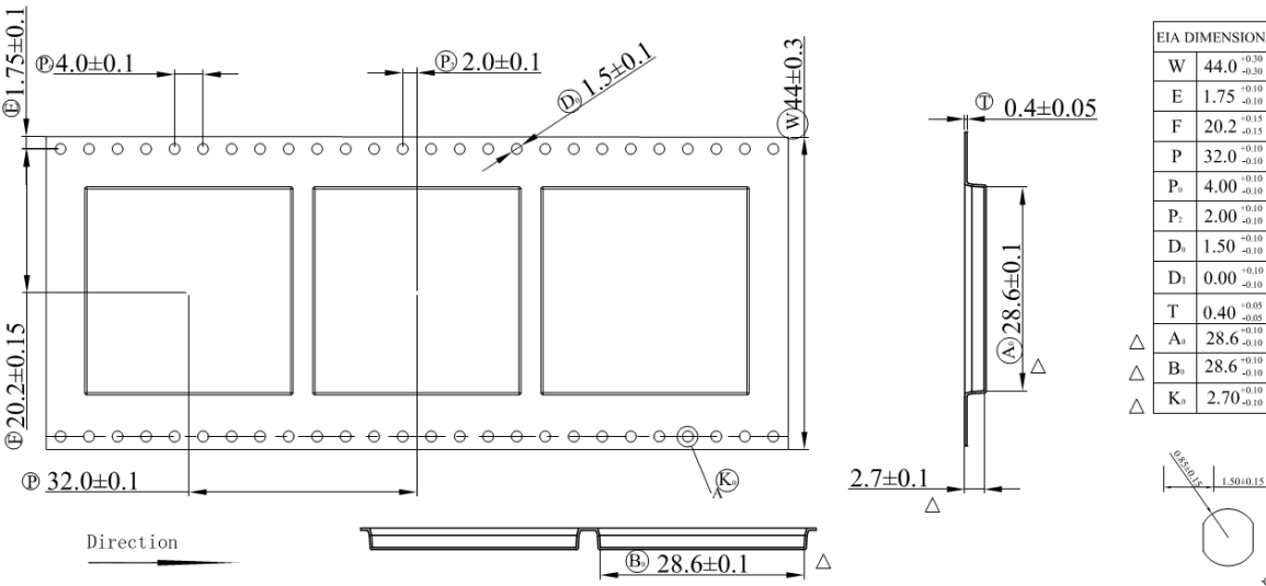
Figure 35: Carrier Tape Detail
