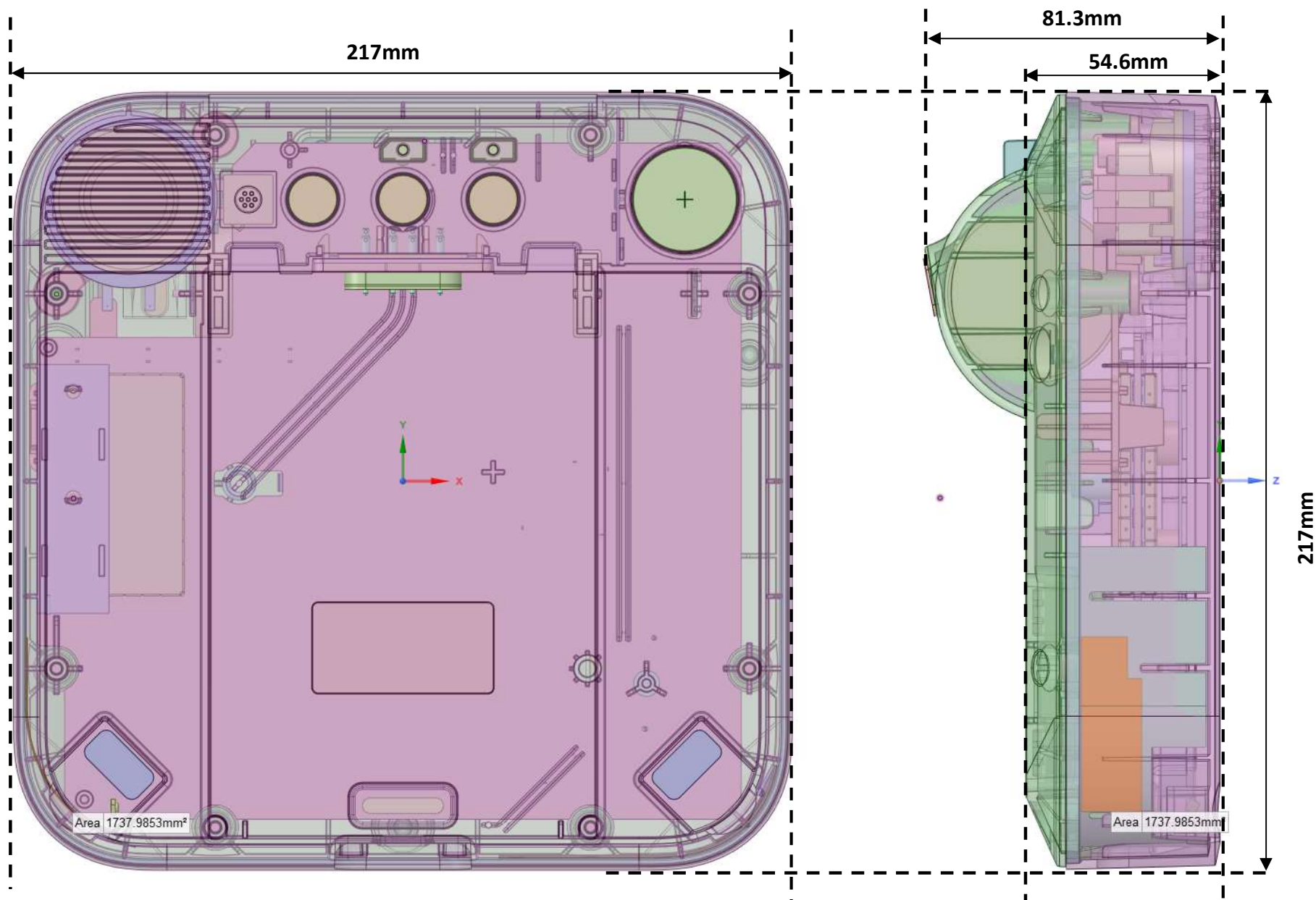
Device Dimension
