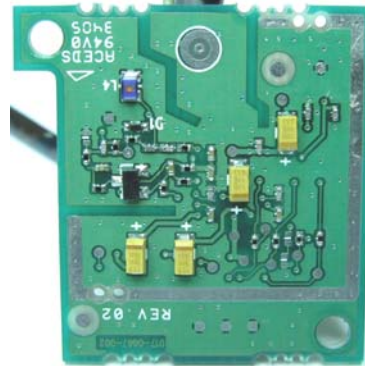
Fig. 2. Bottom view
