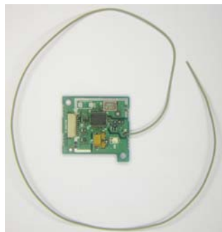
Fig. 5. FMM Top View with antenna attached
