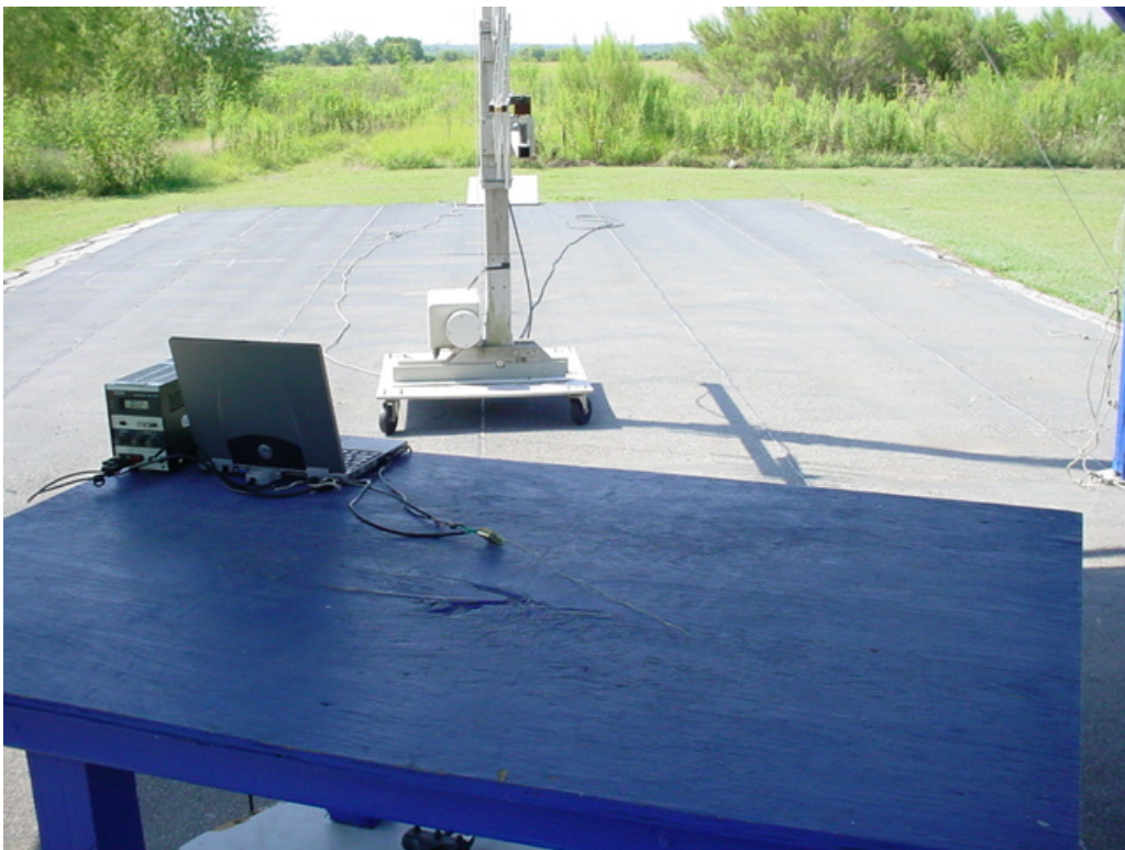
Radiated Emissions at PTI Facility – Rear View
