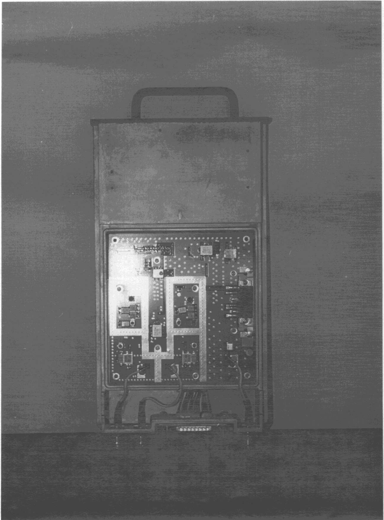
Figure : The Top View(Open and PCB For RCU)
