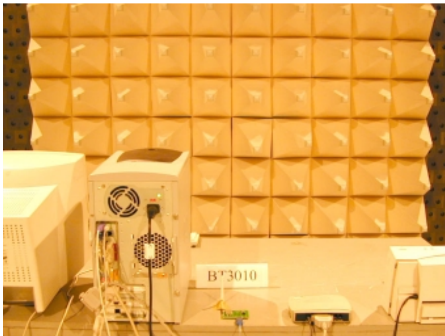
Photo 2: Spurious test set-up photo
