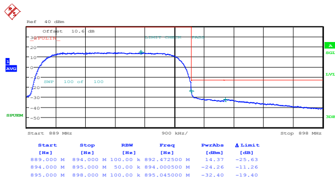
Higher Band Edge Plot on Channel 4458 (891.6 MHz)
