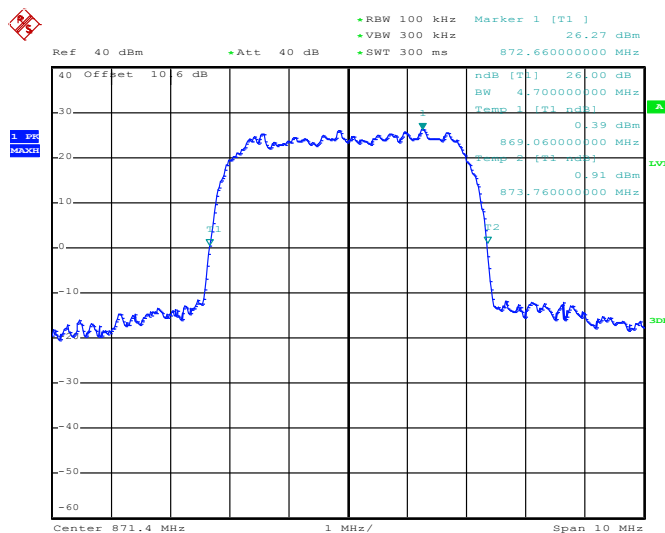
26dB Bandwidth Plot on Channel 4357 (871.4 MHz)
