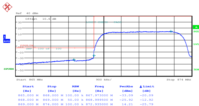
Lower Band Edge Plot on Channel 4357 (871.4 MHz)
