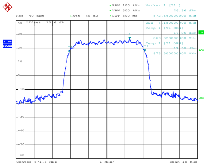
99% Occupied Bandwidth Plot on Channel 4357 (871.4 MHz)
