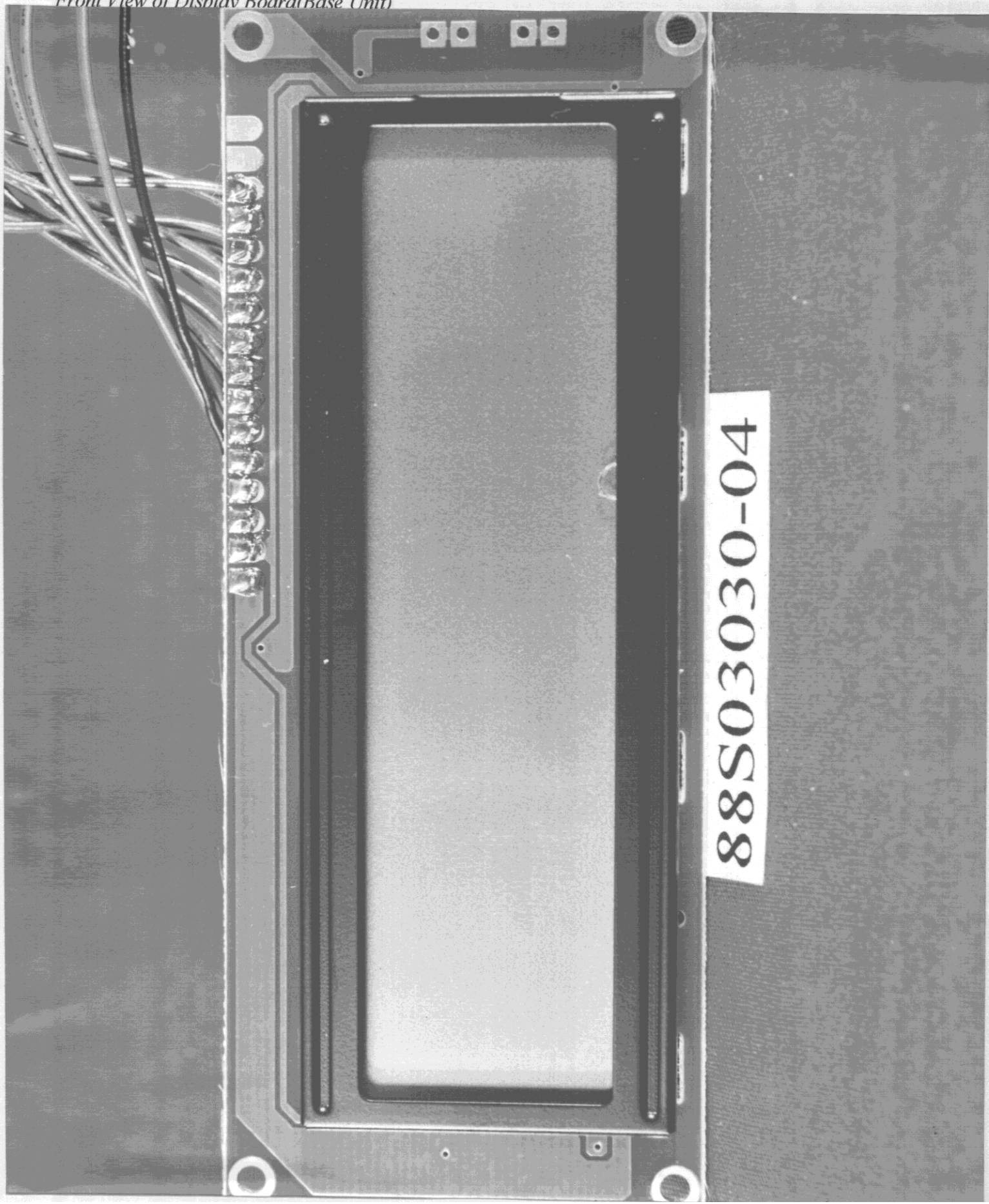
Front View of Display Board(Base Unit)
