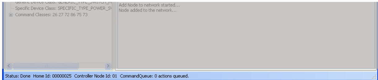
Figure 14. Status Bar
