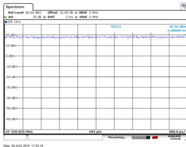
Duty Cycle
