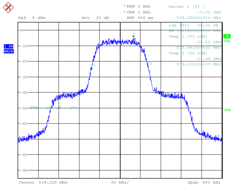
Normal Voltage, -30°C, D2 mode, 539.025 MHz
