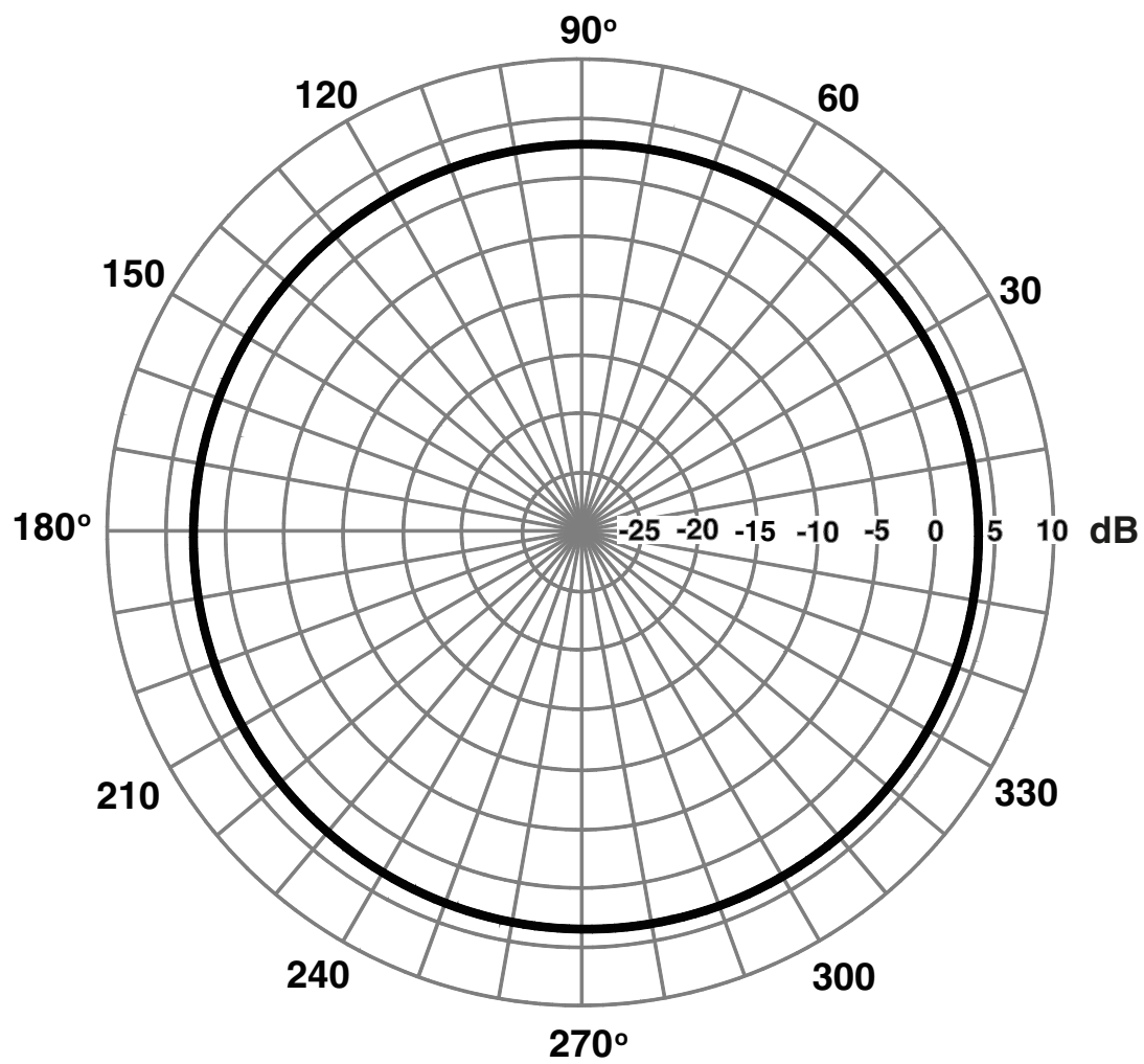
DIPOLE HORIZONTAL PATTERN
