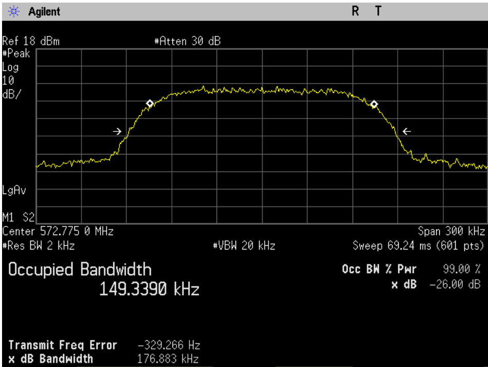
D2 mode: 572.775 MHz, 99% OBW
