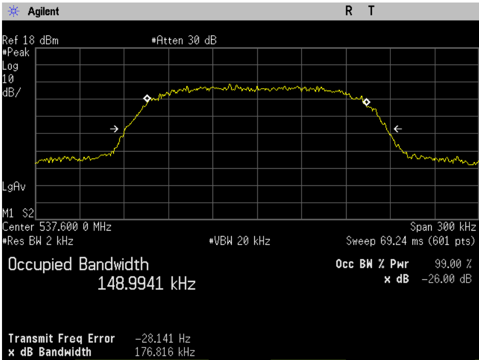
D2 mode: 537.600 MHz, 99% OBW
