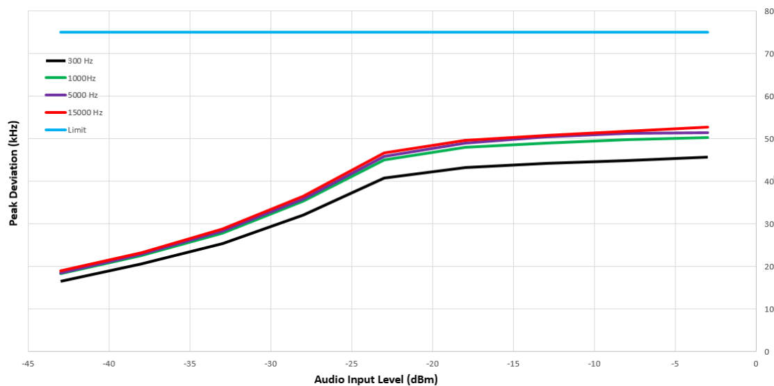
Modulation Characteristics
