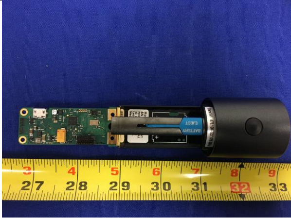
EUT - Cover off
