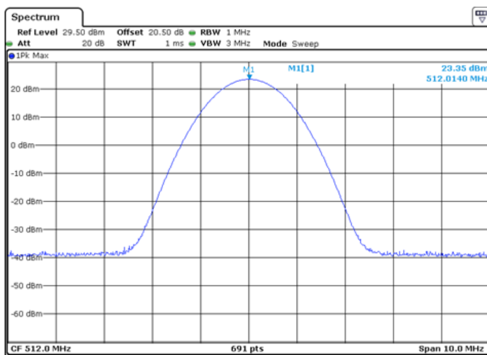
512 MHz Output Power
