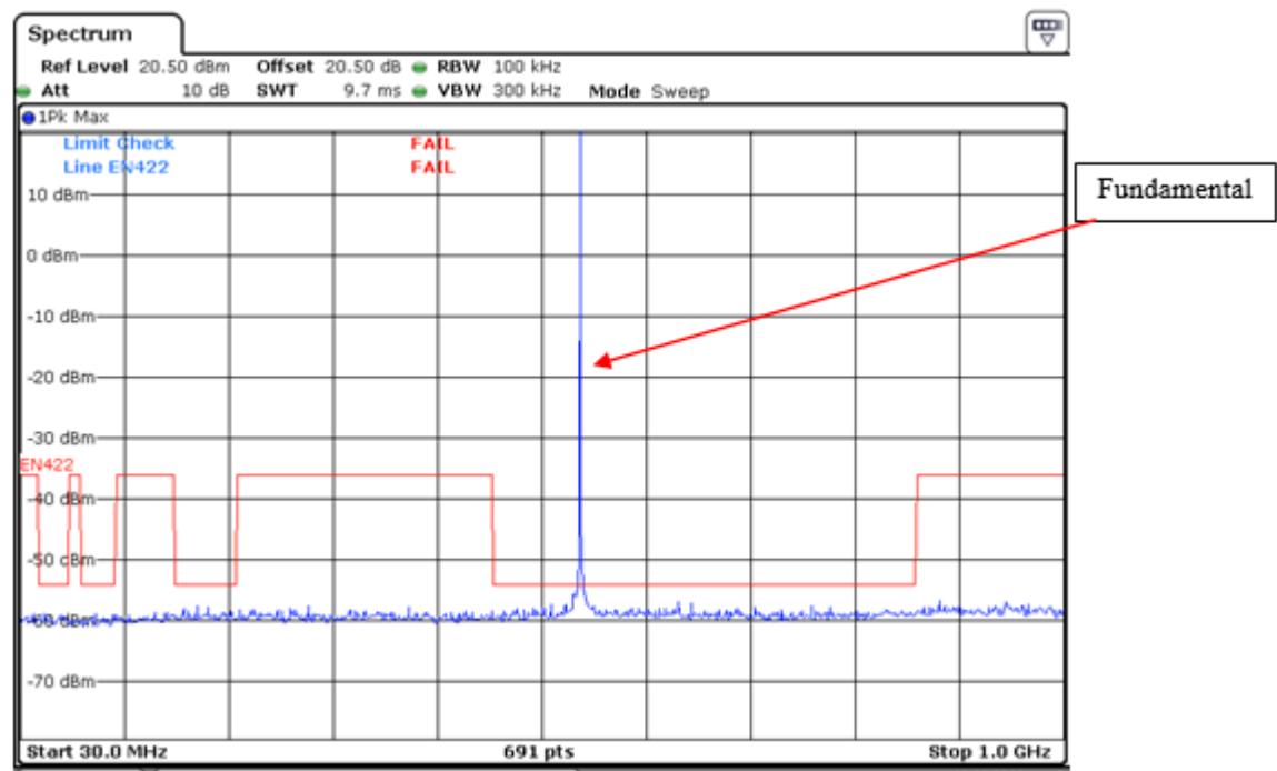
550.4 MHz Spurious Emission below 1 GHz
