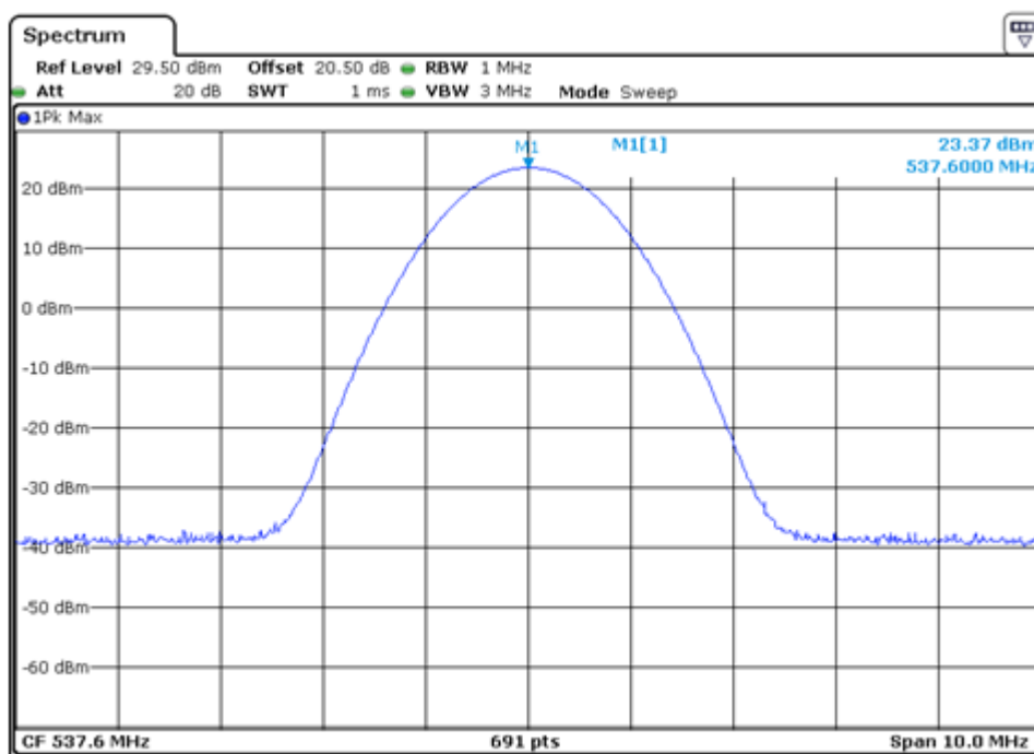
537.6 MHz Output Power
