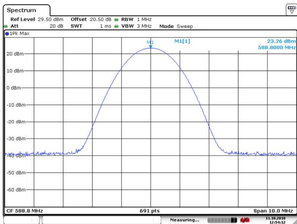
IFBT4 588.8 MHz Output Power
