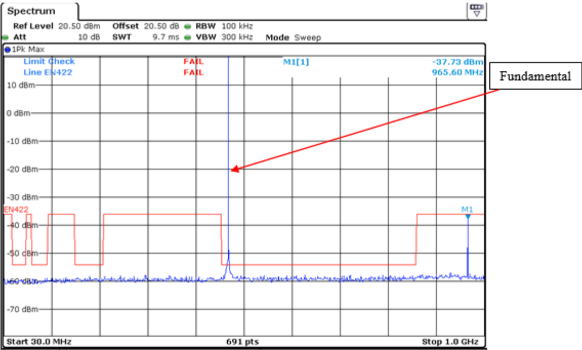
482.9 MHz Spurious Emission below 1 GHz
