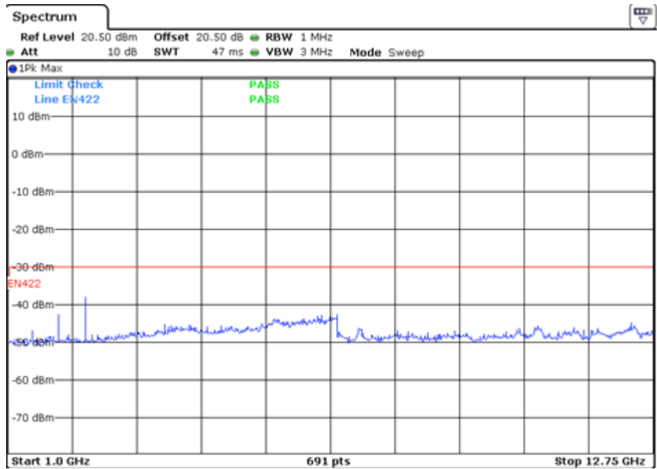
482.9 MHz Spurious Emission above 1 GHz
