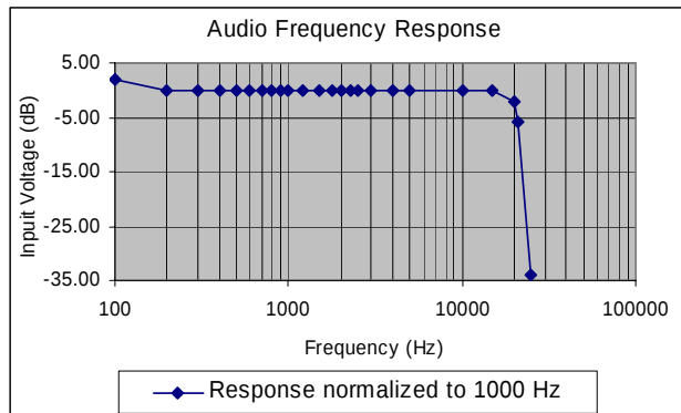
Figure one, Audio Frequency Response Characteristics.
