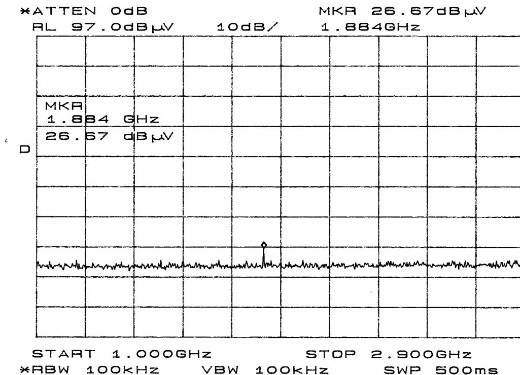
Figure twelve, Radiated emissions from EUT taken in screen room.
