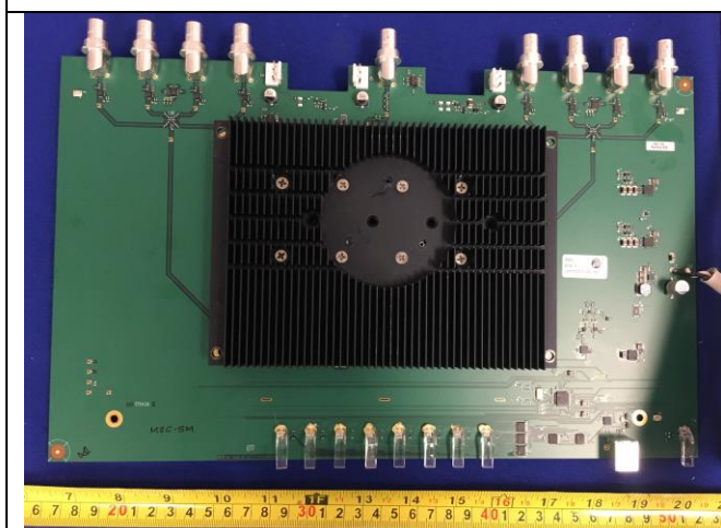
EUT main board Top view without shielding
