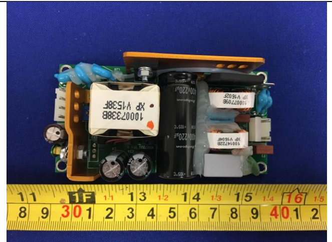
EUT radio board Top view
