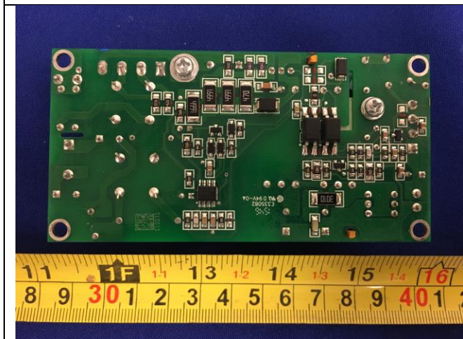
EUT radio board Bottom view
