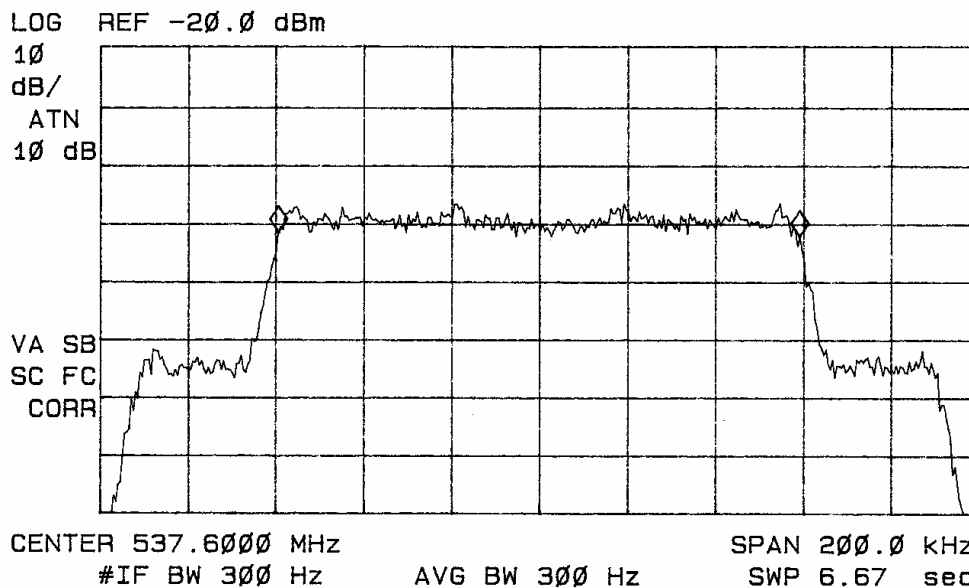
Figure seven Occupied Bandwidth Measurement and Spectral Mask
