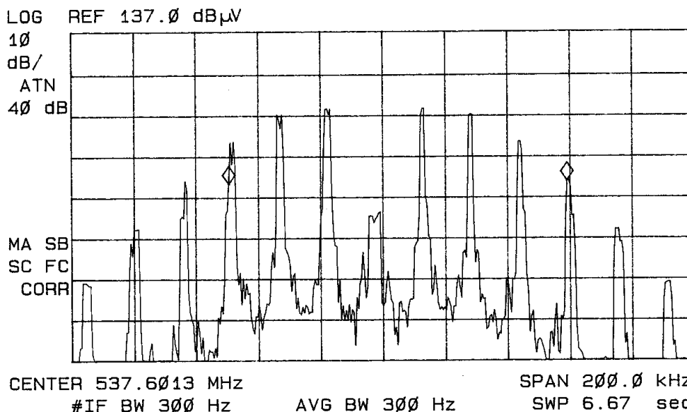
Figure seven(a) Occupied Bandwidth Measurement @ 15,000 Hz
