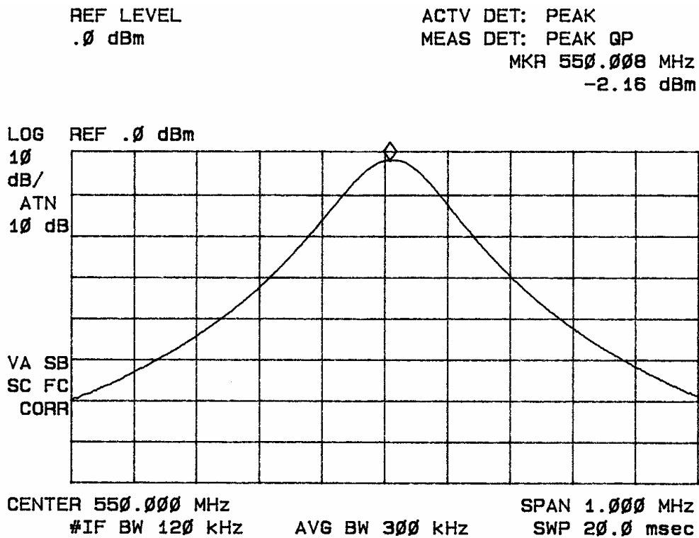
Figure 6 emissions mask
