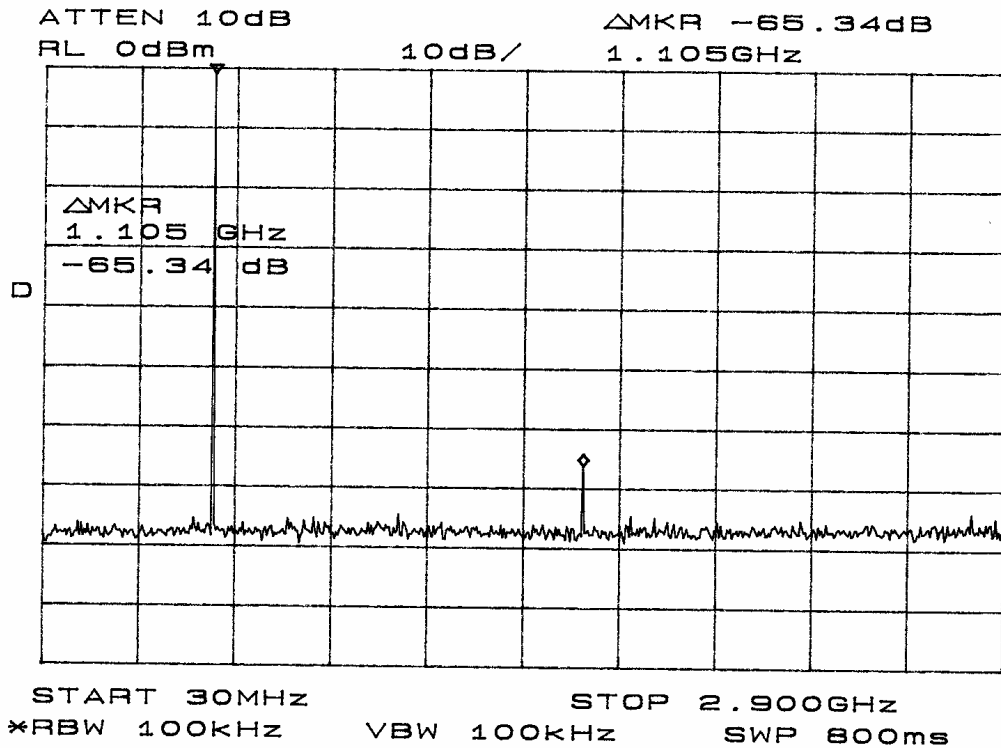
Figure 7 emissions mask
