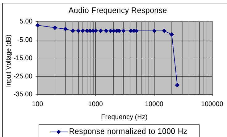
Figure one Audio Frequency Response Characteristics.
