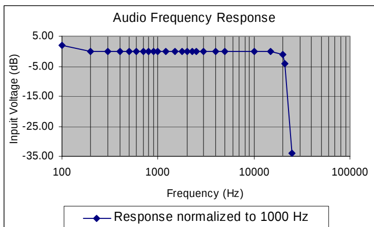
Figure one Audio Frequency Response Characteristics.
