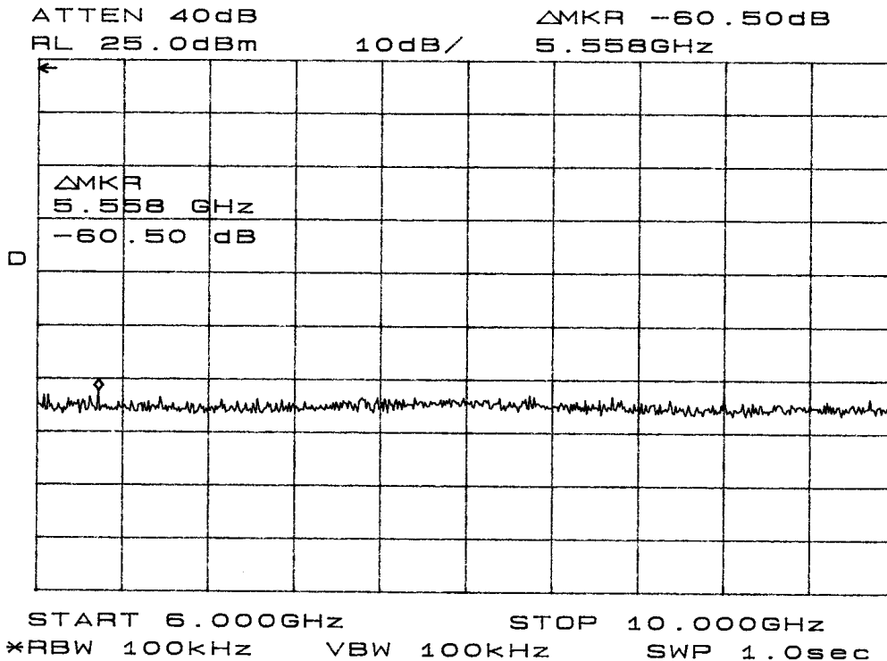
Figure nine emissions mask
