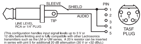
Compatible Standard Unbalanced Line Level Wiring
