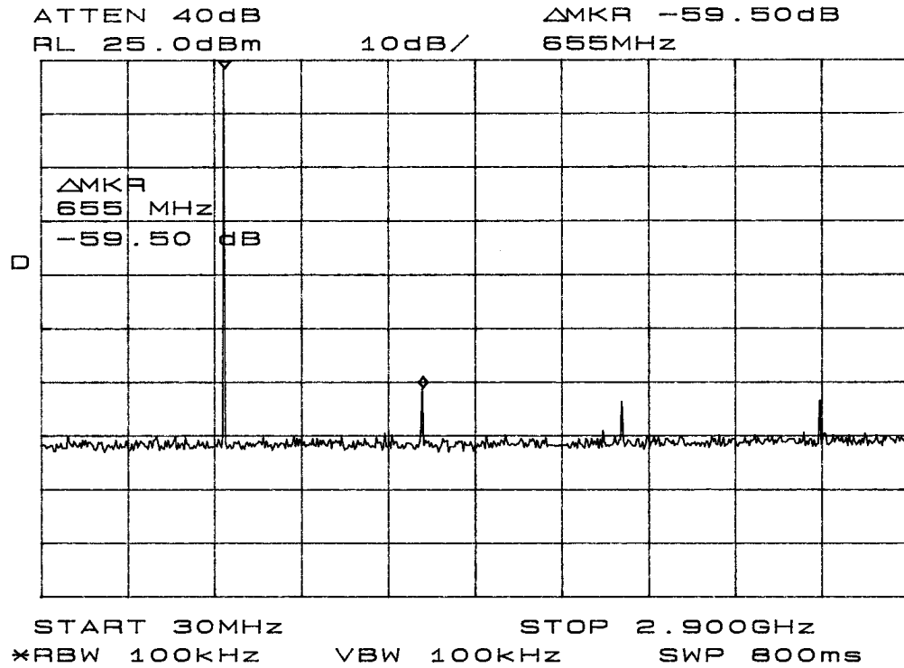
Figure seven emissions mask
