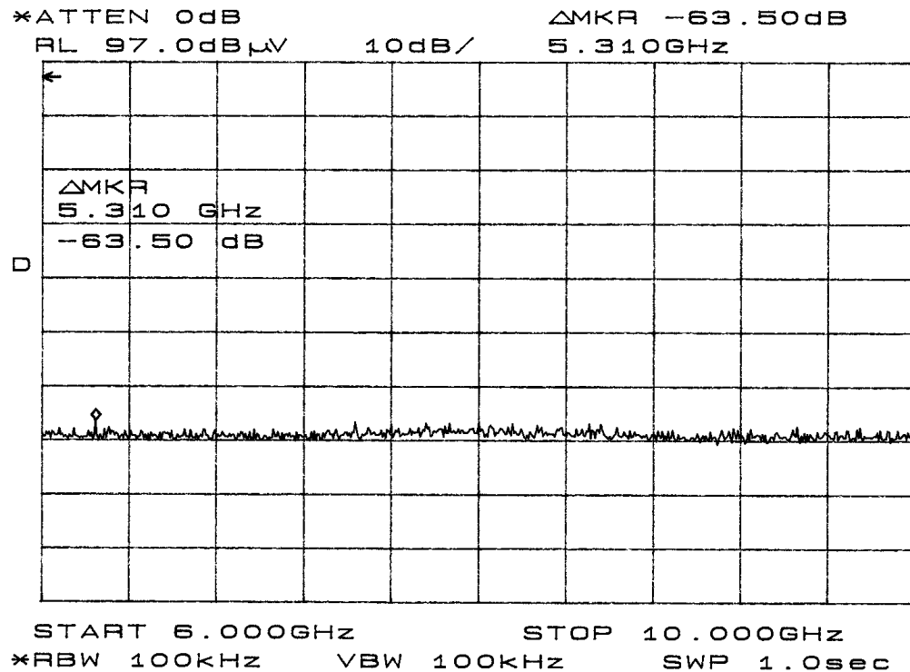
Figure eleven emissions mask
