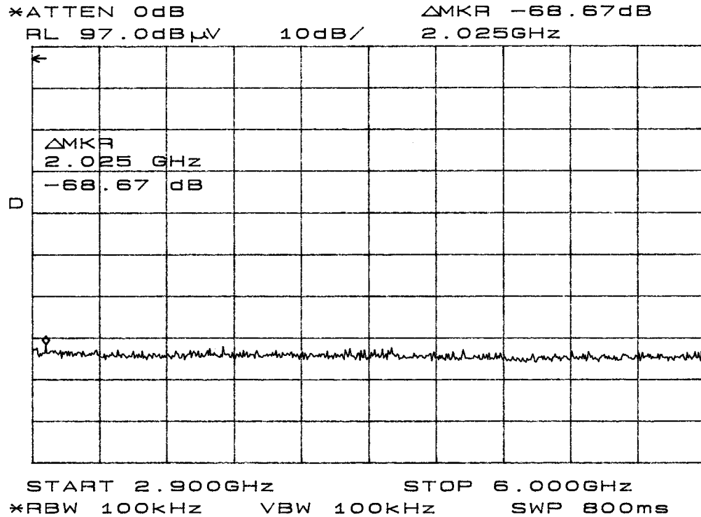
Figure ten emissions mask
