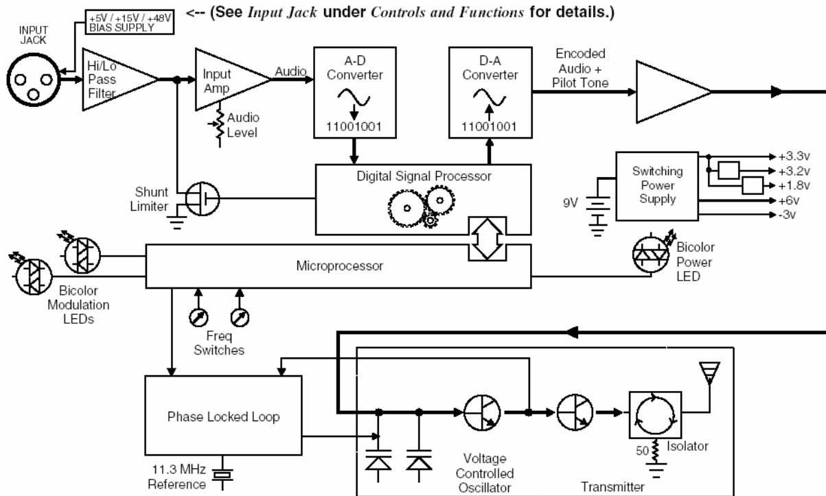
UH400 Block Diagram
