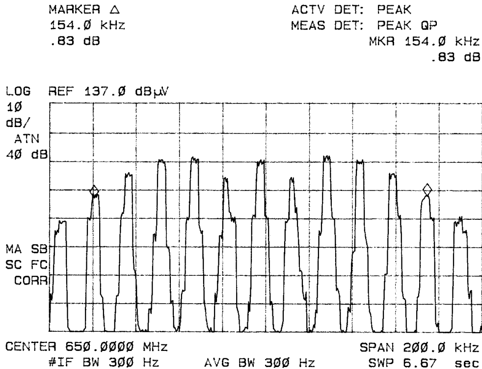
Figure seven(a) Occupied Bandwidth Measurement @ 15,000Hz tone
