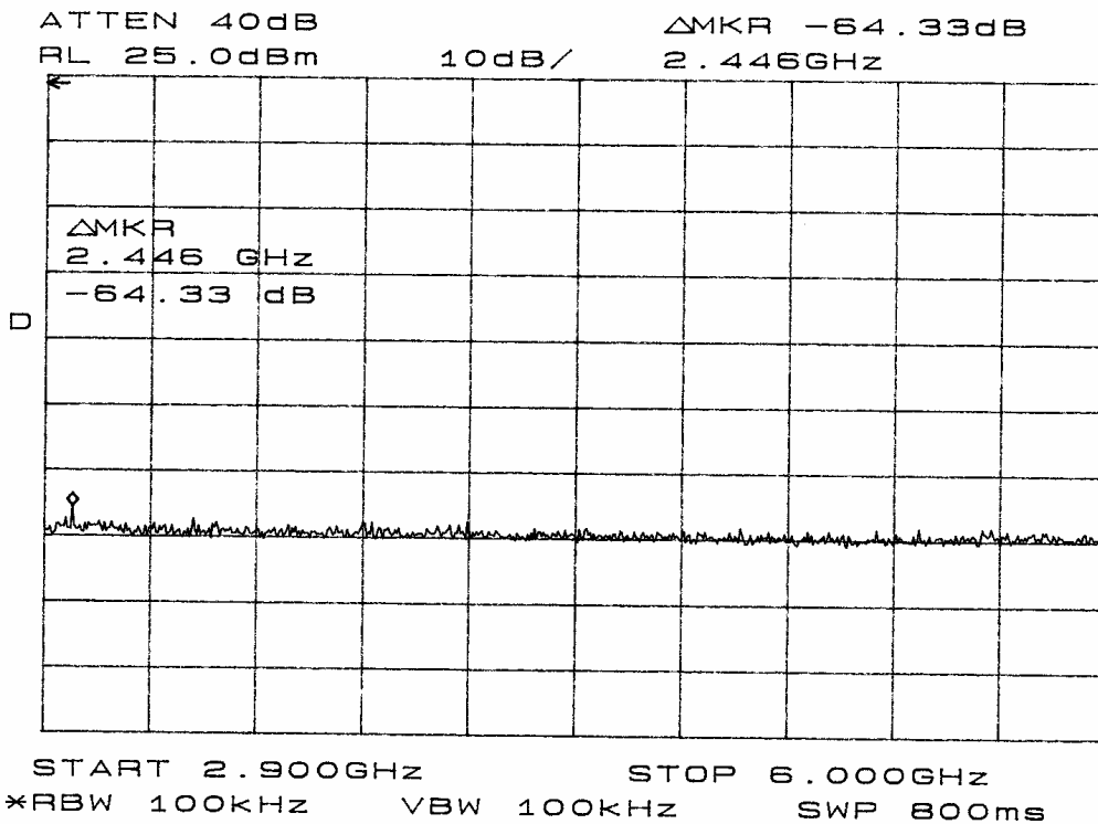
Figure 8 emissions mask
