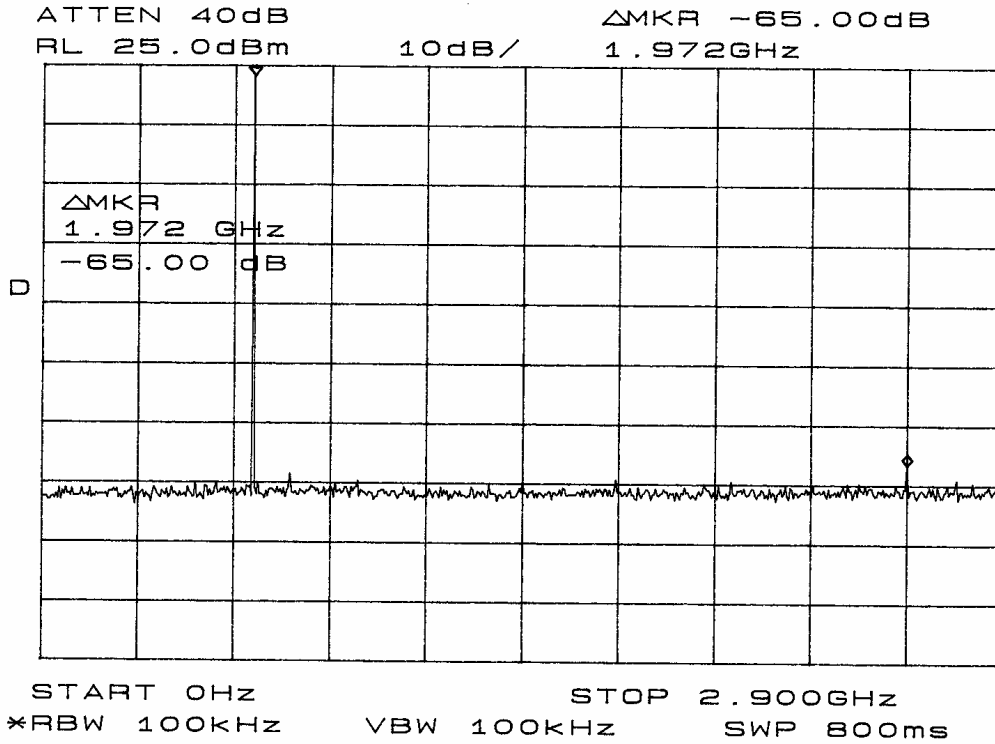
Figure 7 emissions mask
