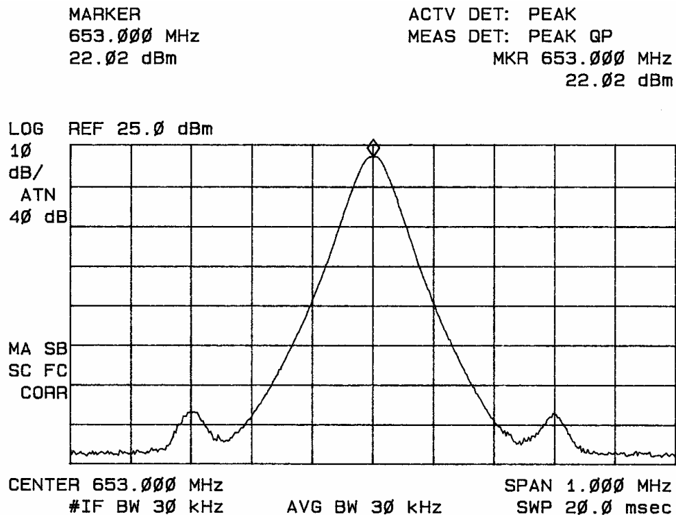
Figure 6 emissions mask
