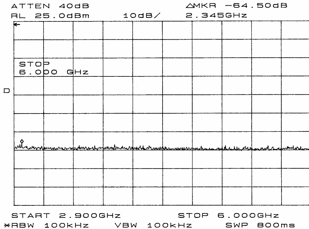
Figure 8 emissions mask
