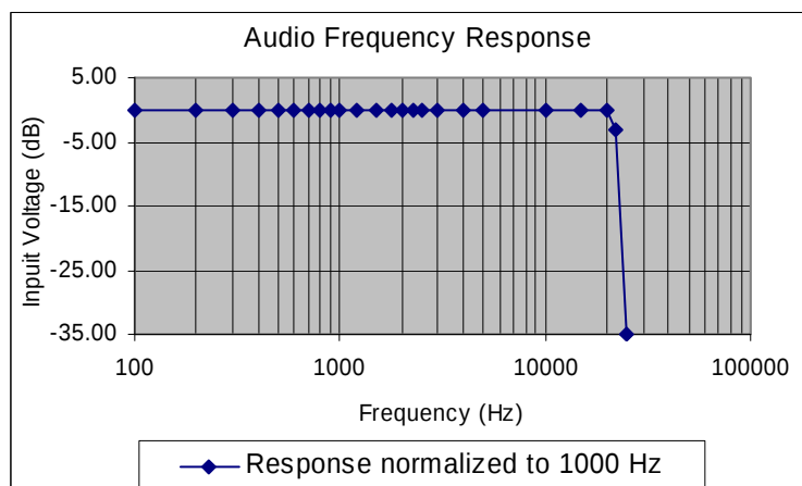
Response of Audio low Pass Filter.
