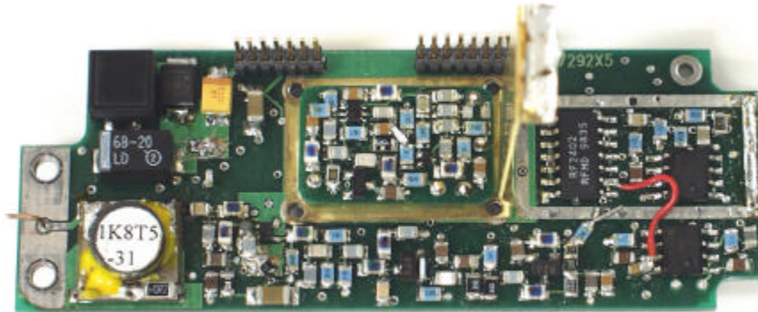
Transmitter Printed Circuit board top.
