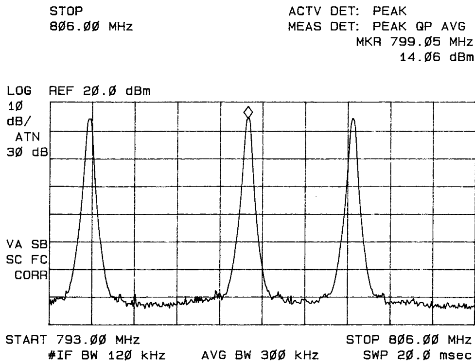
Figure 3: Power Output Block 31
