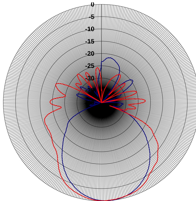
Antenna diagram in [dB] (normalized)
