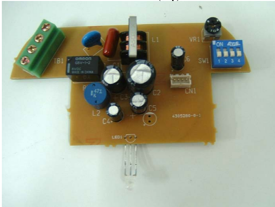
Circuit Board (Top)
