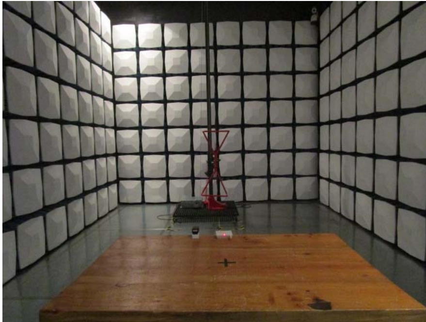
Radiated Emission –Front View (Below 1GHz) (DC 12V)
