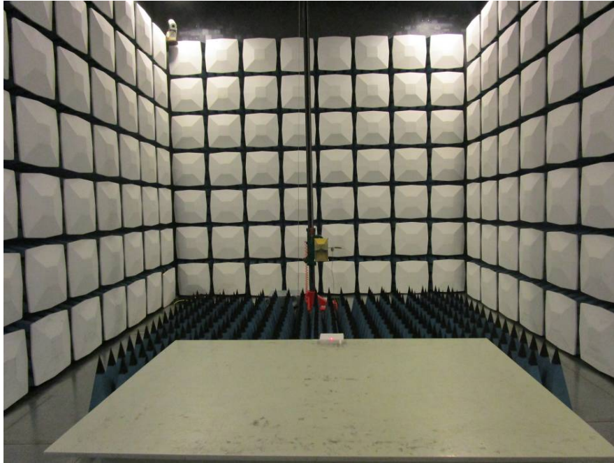
Radiated Emission- Front View (Above 1GHz) (AC 12V)
