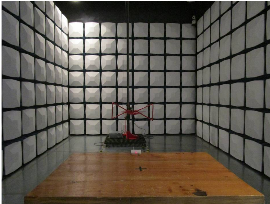
Radiated Emission –Front View (Below 1GHz) (AC 12V)
