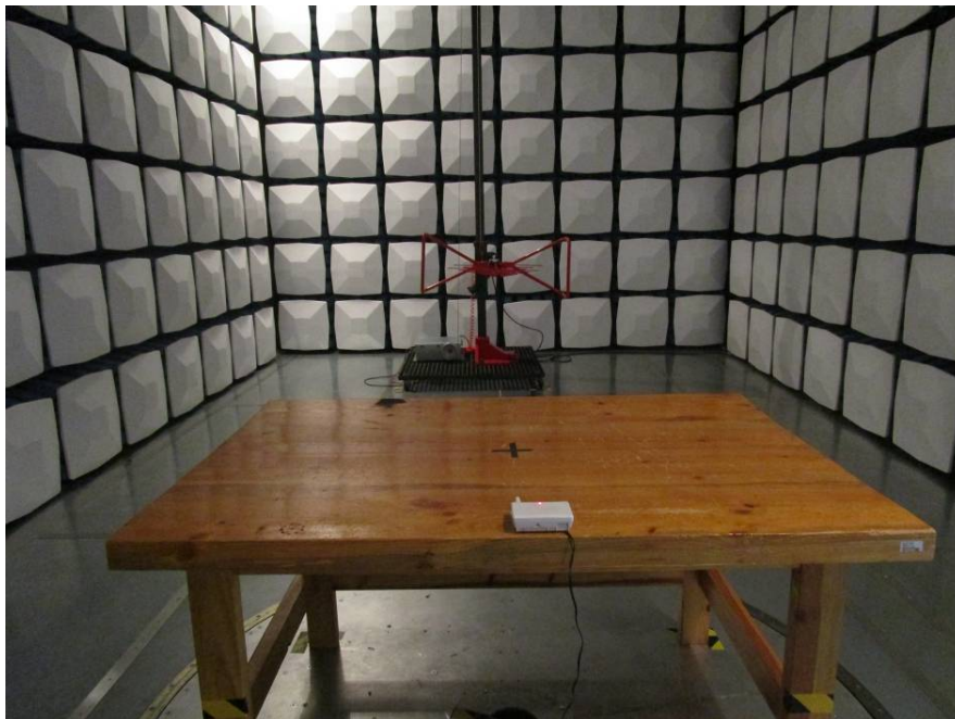
Radiated Emission –Rear View (Below 1GHz) (AC 12V)
