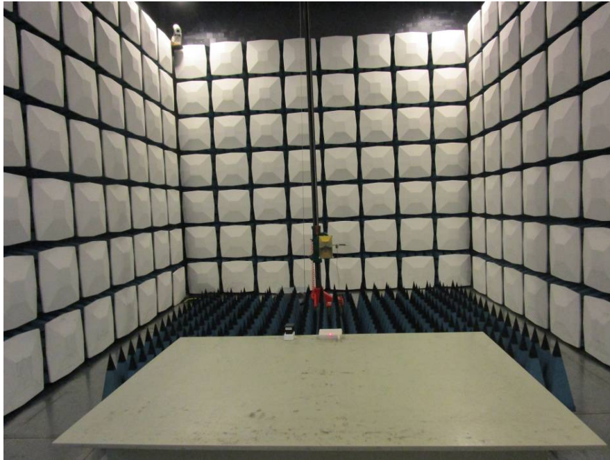
Radiated Emission- Front View (Above 1GHz) (DC 12V)
