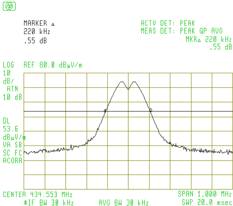
Figure 6.1 Occupied Bandwidth
