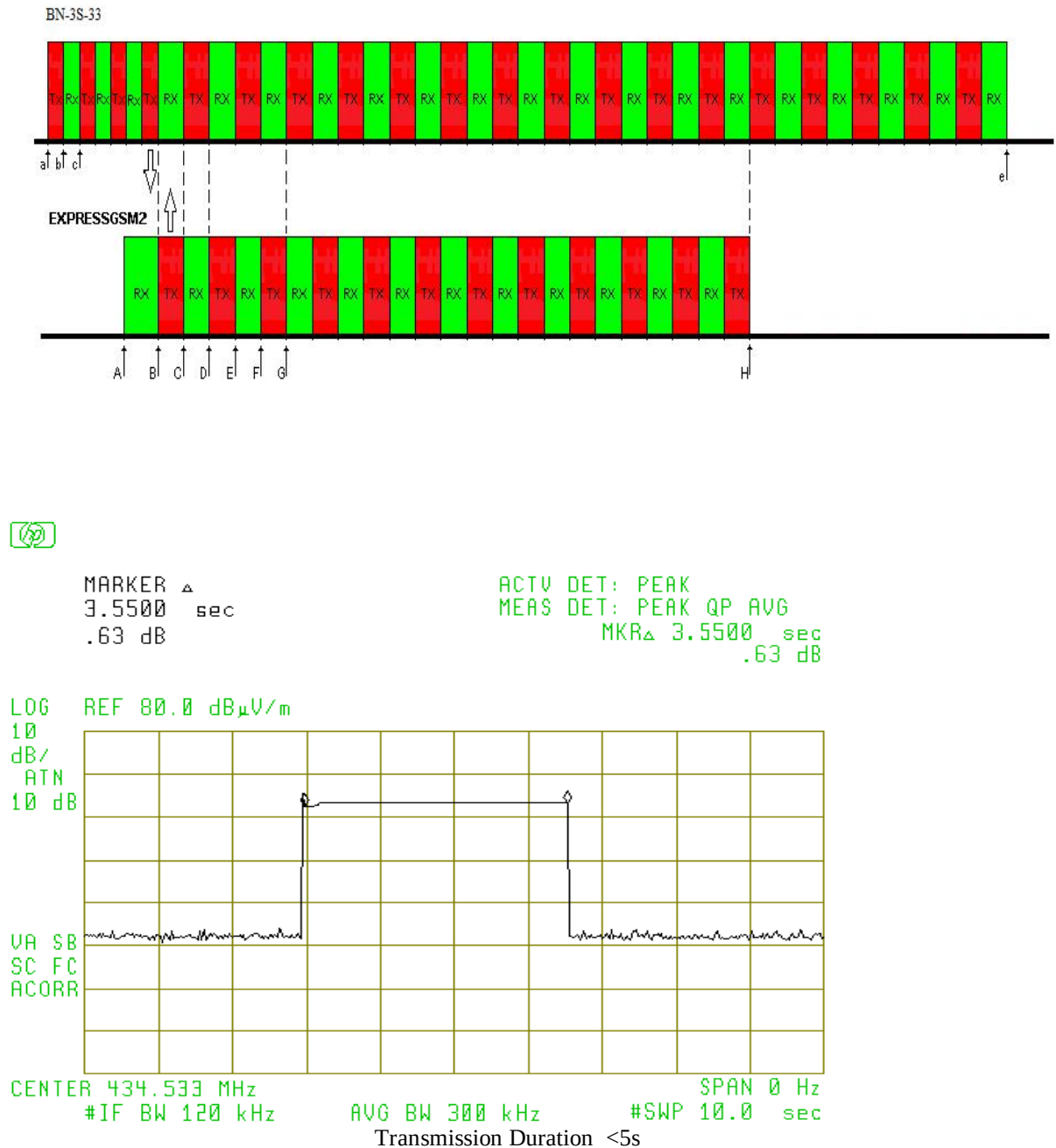
Figure 6.2 Pulse Train Timing
