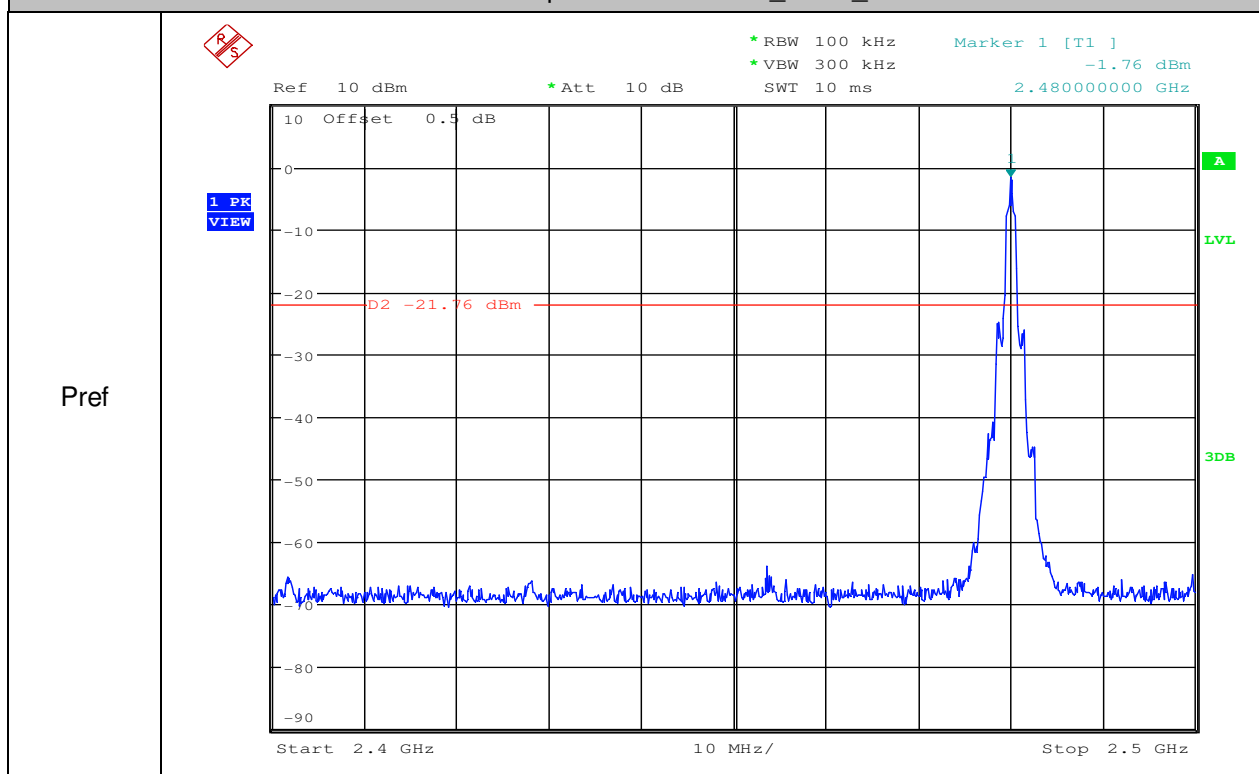
RF Conducted Spurious Emissions 2DH5 2480
